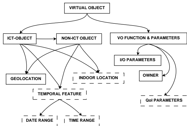
Fig. 2 VO Information Model used. Solid border boxes correspond to elements included in the iCore VO Information Model. Dashed border boxes are new elements introduced by the proposed architecture
