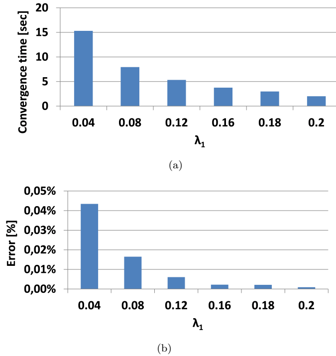
Fig. 11 Convergence time and error on steady state accuracy for different values of \lambda_1 when the algorithm in [31] is used ( \lambda_2 = 0 )
