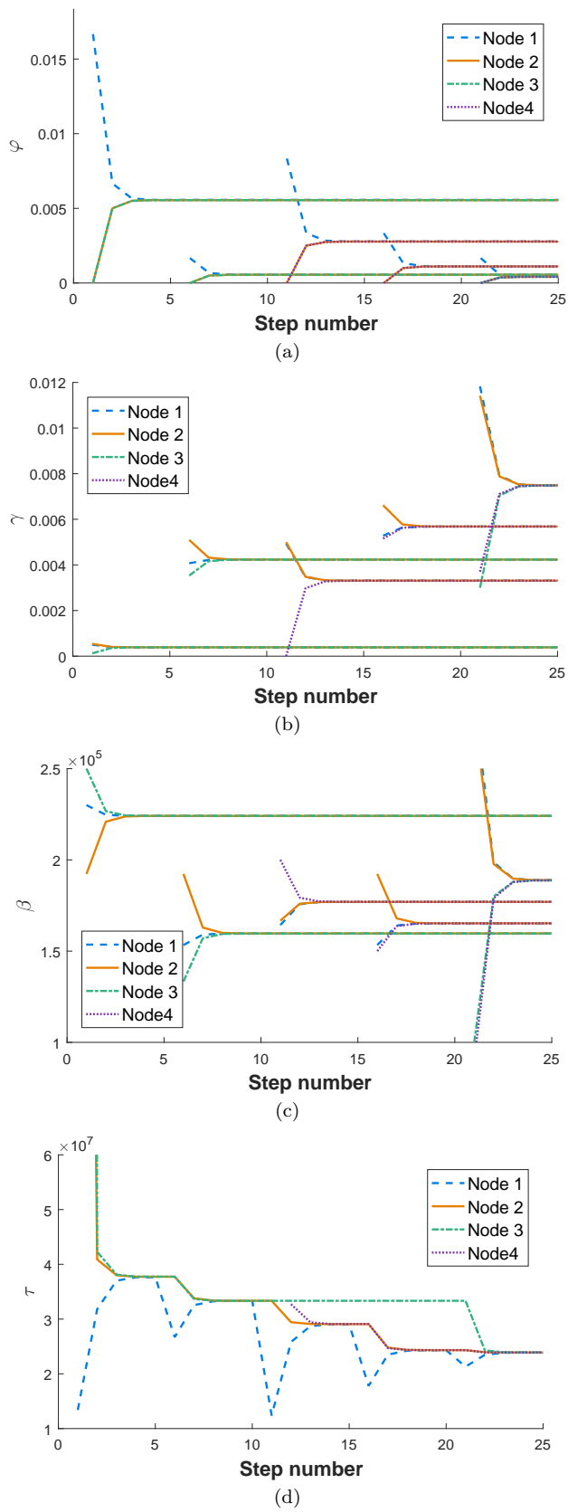
Fig. 5 HVAC management example plot for algorithm convergence
