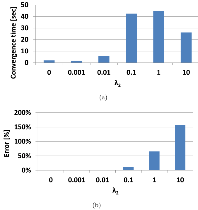
Fig. 12 Convergence time and error on steady state accuracy for different values of \lambda_2 when the algorithm in [27] is used, for a fixed value of \lambda_1 = 0.2
