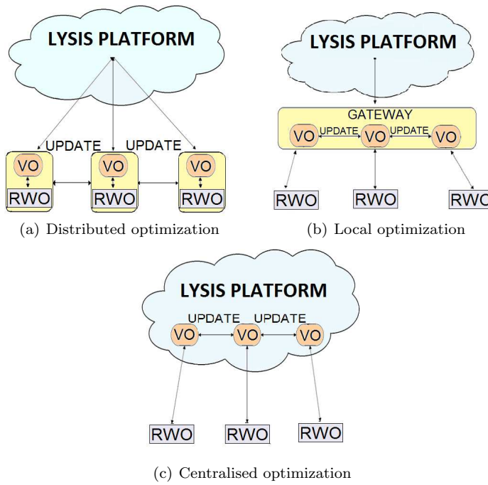
Fig. 4 Location of the proposed algorithm into three typical IoT scenarios with reference to objects' resource allocation
