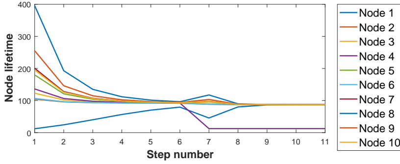
Fig. 7 Example of the ORA algorithm's behaviour when the \delta value increases for node 4 while reaching consensus over a task
