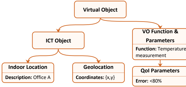
Fig. 3 VO Information Model required to respond to the query for task 1 coming from the Service Level, in the HVAC management example
