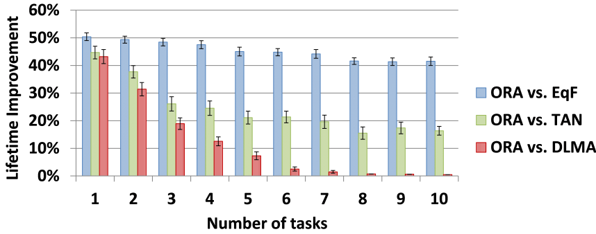
Fig. 8 Average values of percentage improvements in network lifetime for a number of devices equal to 5
