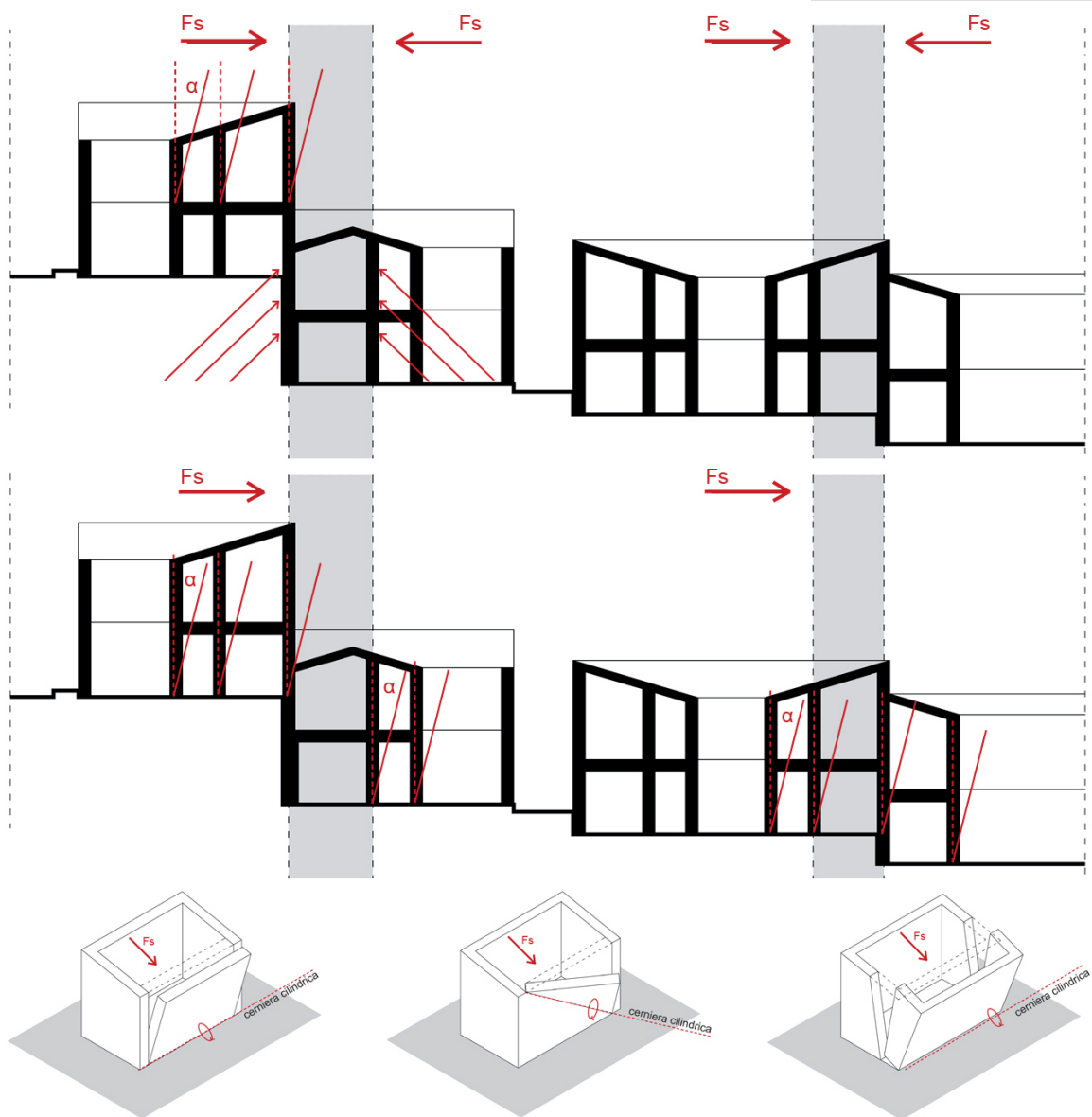
Figure 5. Interpretation of the systemic structural behaviour of the urban aggregate and kinematics of the walls.
