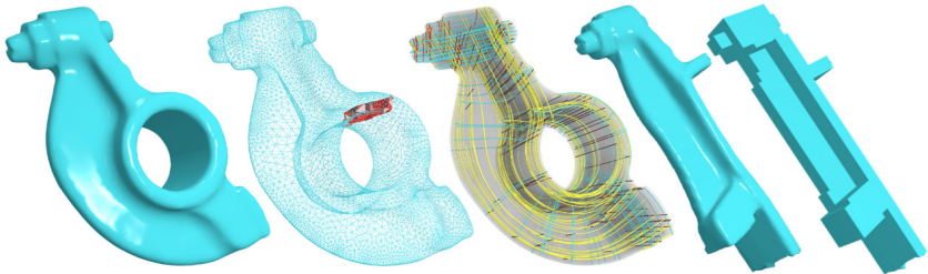
Figure 1.11: Pipeline recap (from [FXBH16]): the input mesh, the cut faces, the computed frame field, the deformed cut mesh and the final polycube.
