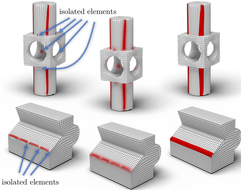
Figure 4.9: Computing hard constraints. Left: D(f) values associated to each facet after the first step; notice, on the top model the isolated high-distortion elements, on the bottom model the isolated low-distortion elements (pointed by the arrows). Middle: D(f) values after the soft propagation. Right: the final constraints resulting from solving the Max Flow - Min Cut formulation, which have filled the interruptions.
