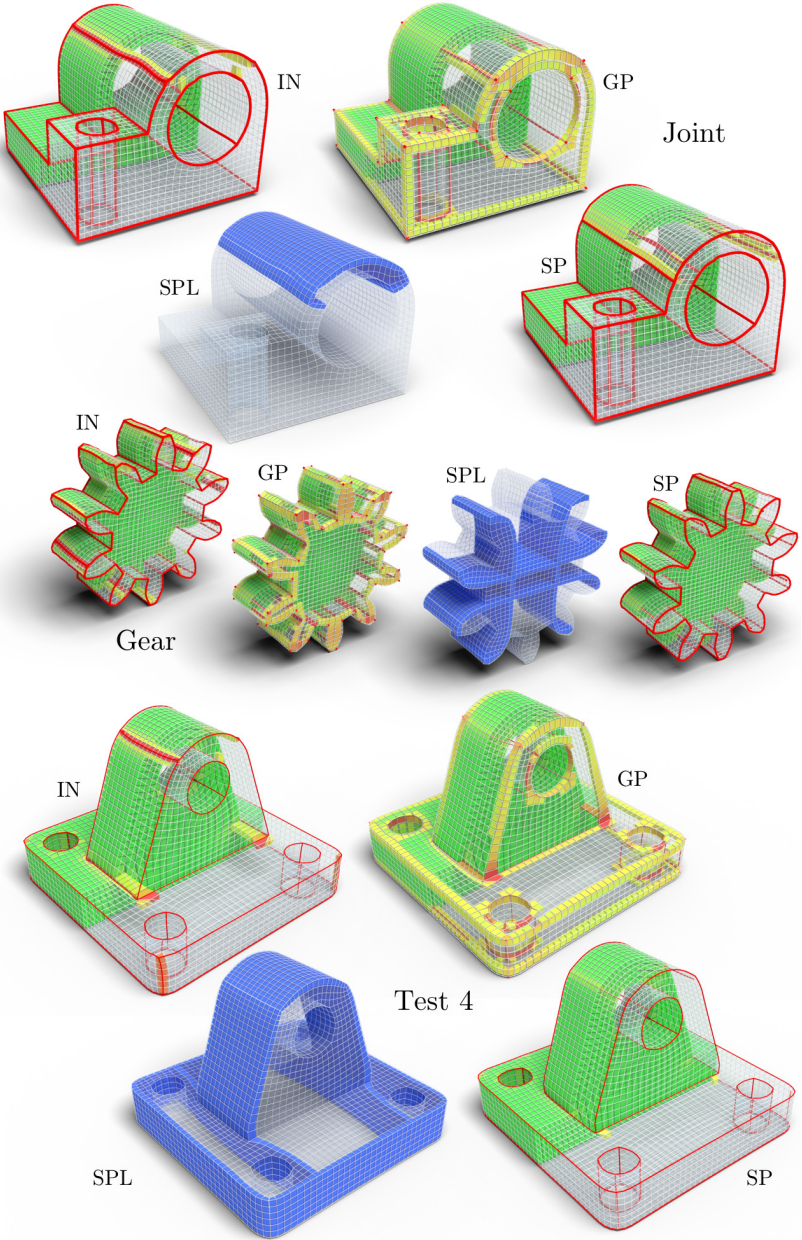
Figure 4.11: Results, pt. 2. For each shape: the input model (IN), the global padding (GP), the new layer, in blue, of the selective padding (SPL) and the final model (SP). Colors indicates quality as described in Figure 4.2.
