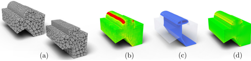
Figure 4.1: The proposed pipeline takes as input a model and its polycube mapping (a); the relative hex-mesh is computed and the surface areas in need of padding are located by analyzing the mapping quality (b); a binary problem is set and solved to find a set of facets to extrude, in order to create a selective padding layer (c); the mapping with the new hex-mesh structure is computed (d).
