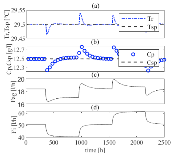
Figure 7. MIMO performances: (a) controlled reactor temperature; (b) controlled ethanol composition; (c) manipulated coolant flow rate; (d) manipulated inlet flow rate.
