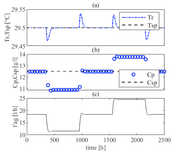
Figure 3. SISO control performances: (a) controlled reactor temperature; (b) ethanol concentration; (c) coolant flow rate.
