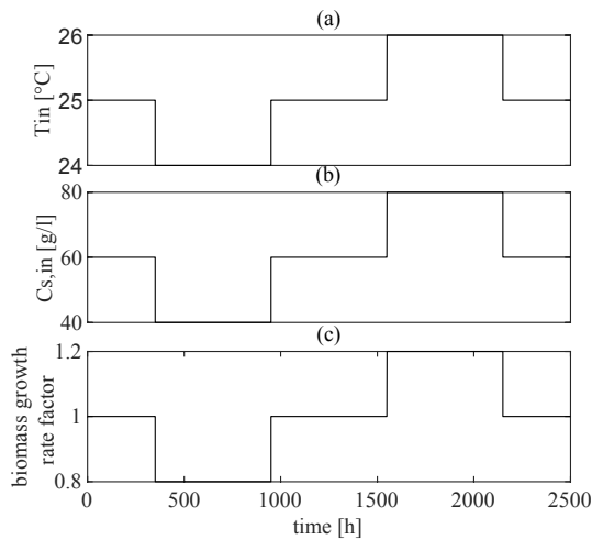
Figure 1. Disturbance trajectories used to analyse the control for the three runs: inlet temperature (a), substrate inlet concentration (b), and biomass growth factor (c).
