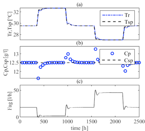
Figure 5. Cascade control performances: (a) controlled reactor temperature; (b) controlled ethanol composition (primary loop); (c) manipulated coolant flow rate.
