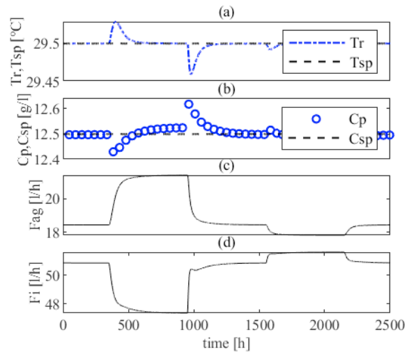
Figure 6. MIMO performances: (a) controlled reactor temperature; (b) controlled ethanol composition; (c) manipulated coolant flow rate; (d) manipulated inlet flow rate.
