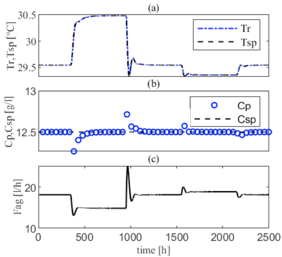
Figure 4. Cascade control performances: (a) controlled reactor temperature (secondary loop); (b) controlled ethanol composition (primary loop); (c) manipulated coolant flow rate.
