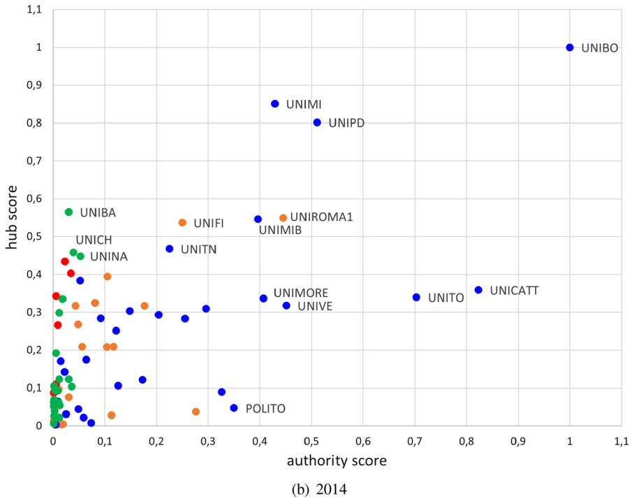
Fig. 4 Scatterplots of hub and authority scores at university level of the 2011–12 and 2014–15 student cohorts according to the Italian macro-areas (blue = north, orange = centre, green = south and red = islands)
