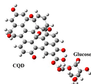
Figure 47. B3LYP/6-31G(p)-optimized structure of CND (referred to as a carbon quantum dot, or “CQD”, by the original authors) interacting with glucose. Reproduced with permission from Sadrollhosseini et al. 33 Copyright 2019 Springer.
