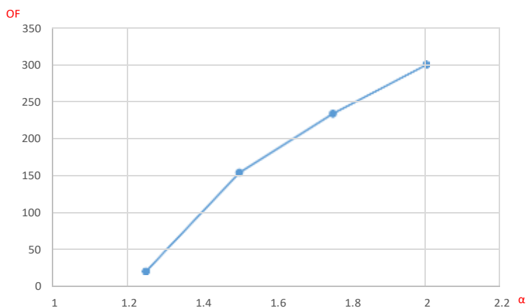
Figure 5: Impact of \alpha on the computational time for a fixed value of m = 5 .
