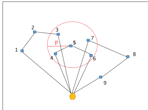
Figure 1: An iteration of LNS Matheuristic. Node 5 has been selected to be removed from the solution. The destroy operator removes all nodes within a certain radius from 5 (included in the red circle), the mathematical model is used to efficiently reconstruct the partial destroyed solution.
