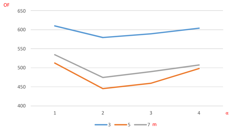
Figure 6: Impact of \alpha on the computational time for different values of m .
