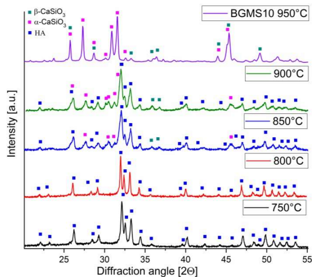
Figure 6. XRD patterns of dense composite samples obtained at different temperatures by SPS from unmilled powders. The pattern corresponding to the sintered glass-ceramic product obtained at 950°C from pure BGMS10 [40] is also reported for comparison.
