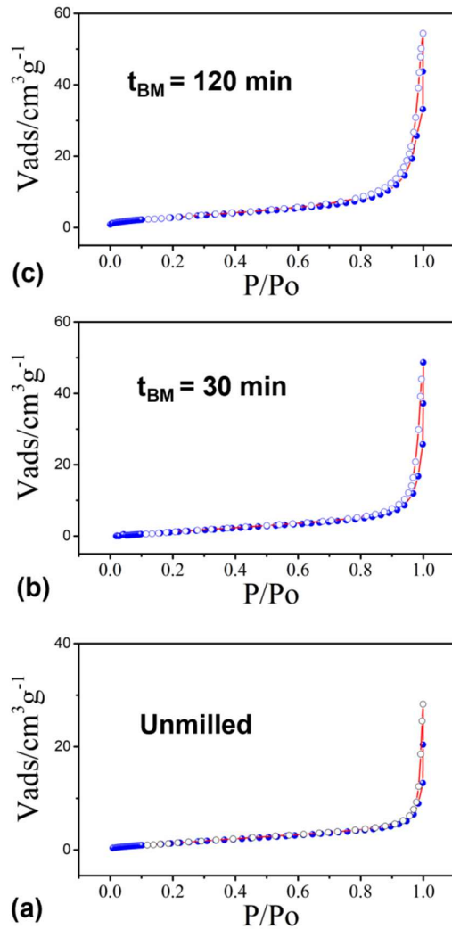
Figure 2. \text{N}_2 physisorption isotherms of the unground (a) sample and, milled for 30 (b) and 120 minutes (c) samples.
