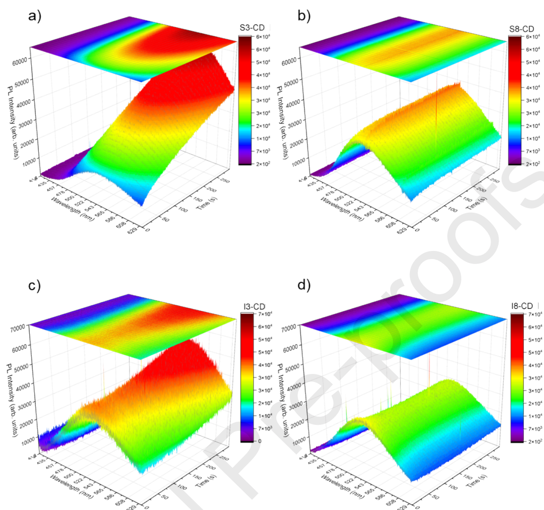
Figure S9. 3D plots of irradiation effects on S3-CD (a) and S8-CD (b), I3-CD (c), I8-CD (d). Laser irradiation was performed with 405 nm CW light focused on the samples with a microscope objective (power 5 \mu W, spot diameter 6.4 \mu m).
