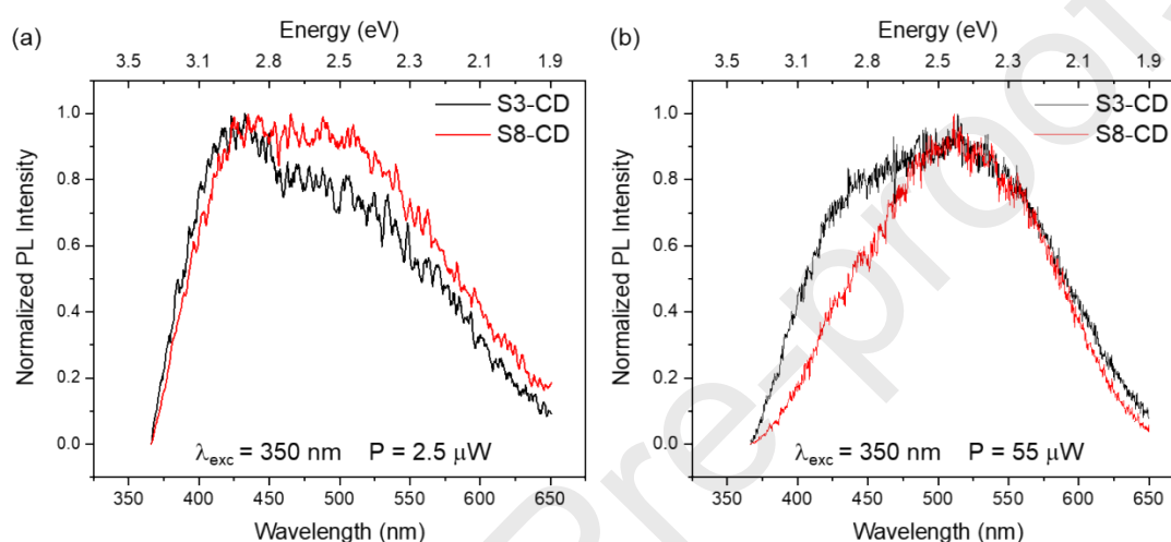
Figure 6. Normalized PL spectra of hybrid samples under 350 nm irradiation at 2.5 \mu W (a) and 55 \mu W excitation power (b).
