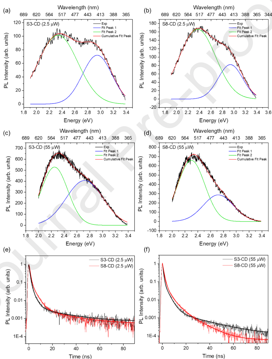
Figure S1. Gaussian deconvolution of hybrid samples irradiated at 350 nm at low (2.5 \mu W) and high (55 \mu W) excitation power and corresponding decay time plots with relative fits (details in Table S1 and S2). Jacobian factor for the correction of the PL intensity was applied in all spectra. The decay time was recorded on the overall emission spectrum.
