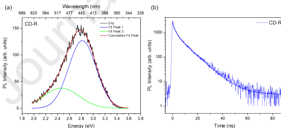
Figure S8: Spectral deconvolution by gaussian bands of CD-R sample (a) and data fit of its decay time (b) excited at 350 nm. Details in Table S1 and S2. The decay time was recorded on the overall emission spectrum.
