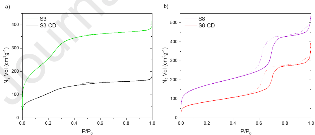
Figure S5. N_2 adsorption-desorption curves at 77 K of S3-CD (black line) and S3 (green line) samples (a), S8-CD (red line) and S8 (purple line) samples (b).
