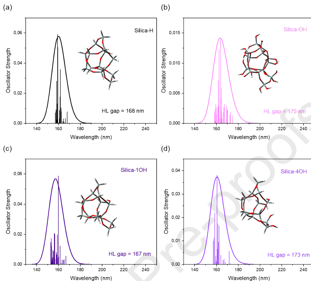
Figure S10: Calculated optical absorption features of isolated emitting center models (simplified stick representation: white stick = H atom, dark grey stick = C atom, red stick = O atom).
