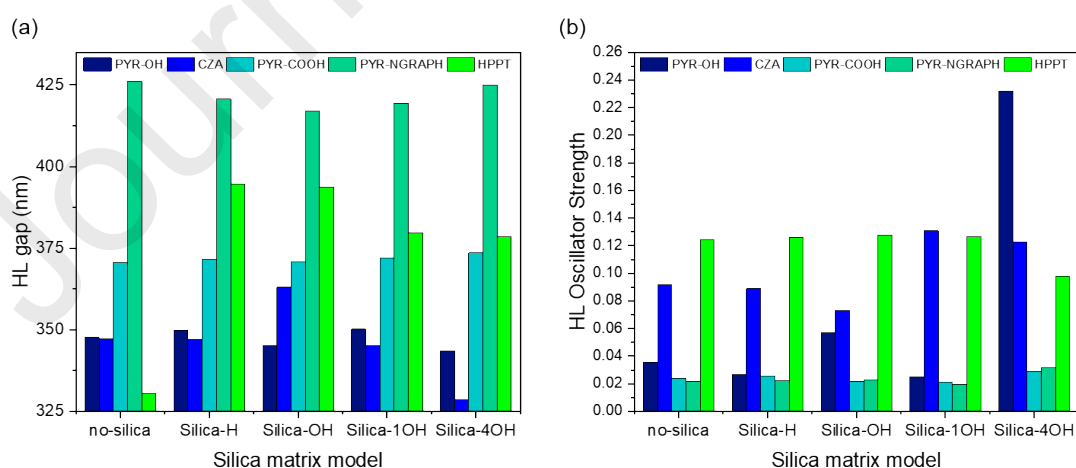
Figure S11: HL gap (left) and oscillator strength (right) for the different model structures without silica, or in presence of fully H terminated, fully OH terminated silica, and partially OH terminated (1 OH or 4 OH) silica models.
