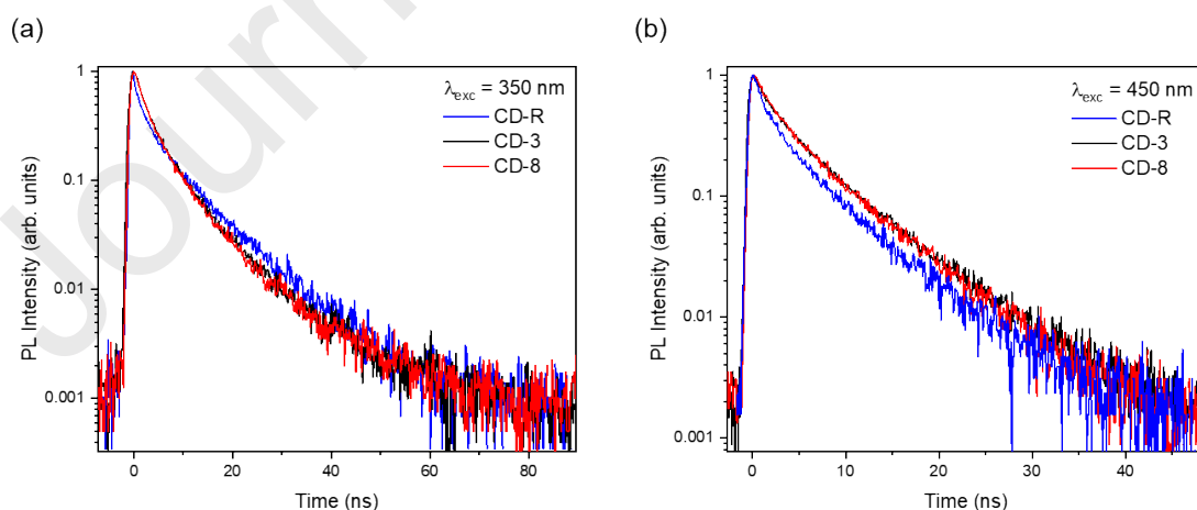
Figure S6. Decay time plots in the 100 ns range of CD-R, CD-3 and CD-8 excited at 350 and 450 nm. The decay time was recorded on the overall emission spectrum.
