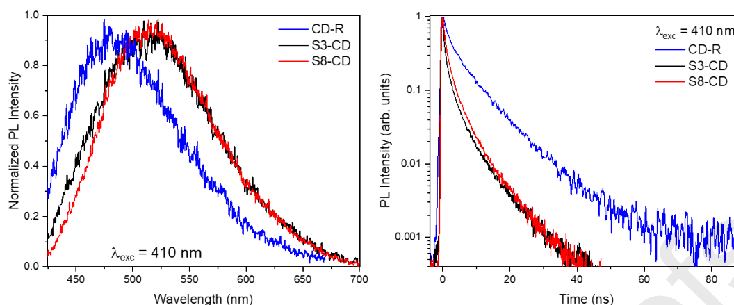
Figure S7. Comparison of TR-PL spectra excited at 410 nm with an excitation power of 55 \mu W, and the relative decay time plots in the 100 ns range for CD-R and 50 ns range for the hybrids S3-CD and S8-CD. The decay time was recorded on the overall emission spectrum.
