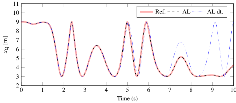
Fig. 8 Case 2: effect on displacement x_Q of the slider of the parameter selection of augmented Lagrangian methods.
