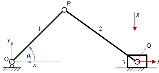
Fig. 1 Slider-crank mechanism used as a benchmark problem.
