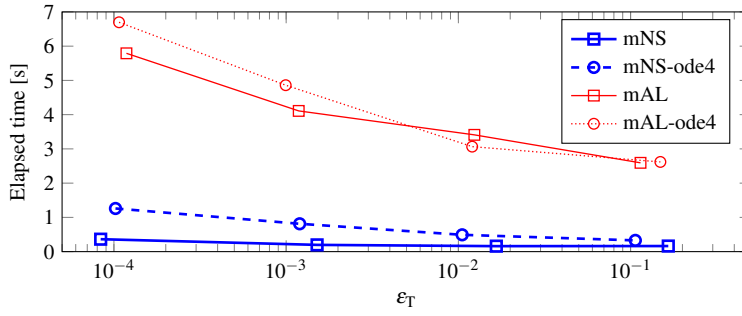
Fig. 9 Elapsed time in the solution of case 2 as a function of the precision \varepsilon_T delivered by mAL and mNS methods.
