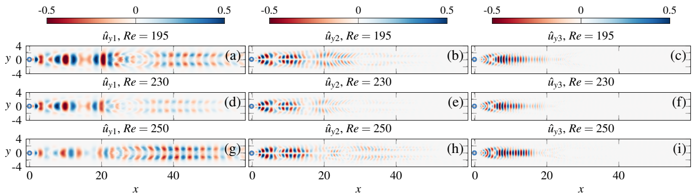
FIG. 17. Modal form of (a,d,g) first, (b,e,h) second and (c,f,i) third harmonic, for Da = 9 \times 10^{-4} and Re = 195 (top), Re = 230 (center) and Re = 250 (bottom), rescaled with the corresponding maximum absolute value.
