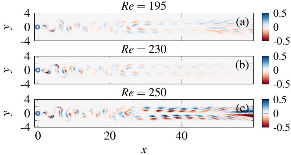
FIG. 12. Spanwise ( z ) component of vorticity (rescaled with its maximum absolute value) from the linearized simulations at t = 100 and Da = 9 \times 10^{-4} : (a) Re = 195 , \beta = 1.56 , (b) Re = 230 , \beta = 1.5 and (c) Re = 250 , \beta = 1.5 .
