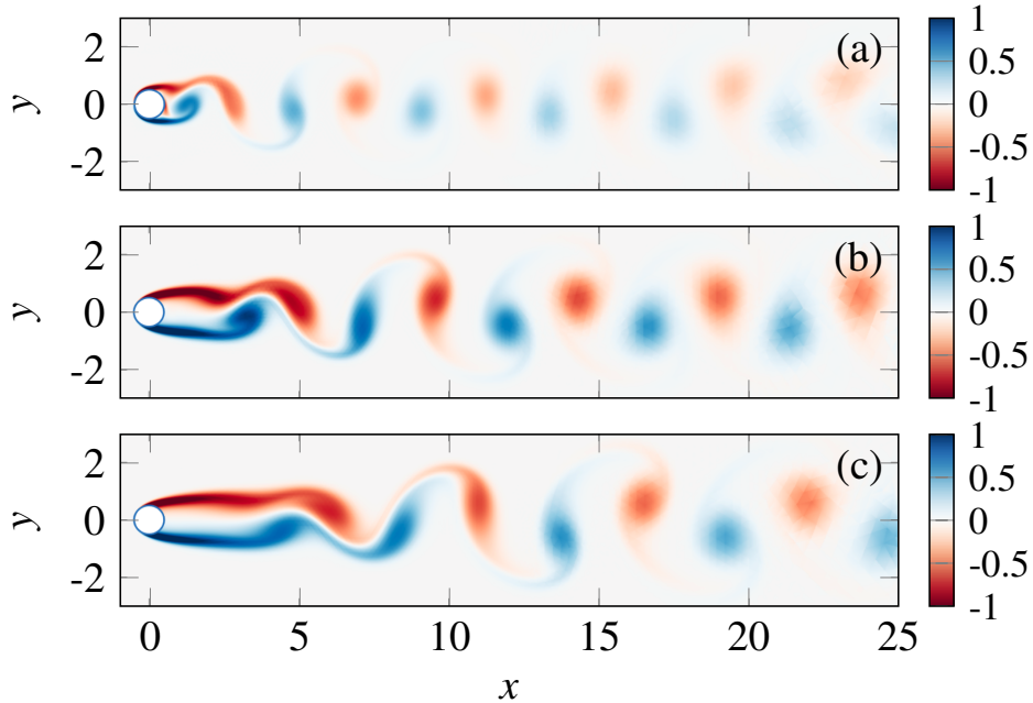
FIG. 4. Spanwise base-flow vorticity snapshots for (a) Re = 215 , Da = 1 \times 10^{-4} , (b) Re = 200 , Da = 2 \times 10^{-3} and (c) Re = 215 , Da = 3 \times 10^{-3} , normalized with the corresponding maximum absolute value, i.e. (a) \max(|\omega_z|) = 27.3 , (b) \max(|\omega_z|) = 8.3 , (c) \max(|\omega_z|) = 6.1 .
