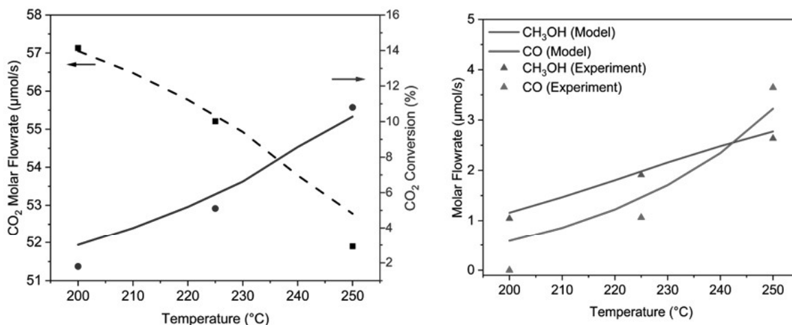
Figure 4- CO_2 conversion (a) and product outlet molar flowrates (b) as a function of temperature. All these experiments/model data are measured/computed at P=30 bar. T=250 °C, GHSV=7,000 h^{-1} , inlet pH_2 , pCO_2 , pN_2=19.9 , 6.7, 2.9 (bar) respectively, whenever it is not varied. Symbols represent experimental data points. Lines represent microkinetic model predicted data points. Color codes: Blue- CO_2 conversion; Black, Green, Red- reactor outlet CO_2 , CH_3OH , CO molar flow rates.
