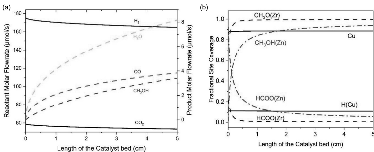
Figure 6 (a)- The gas phase and (b) catalyst surface species as a function of catalyst bed length, obtained from the microkinetic model. In the gas-phase profile, \text{CO}_2 and \text{H}_2 have their scale on the left and the remaining species have their scale on the right. In the surface species plot, solid lines represent the species on Cu, dashed lines represent the species on \text{ZrO}_2/\text{Cu} interface and the dot-dashed lines represent the species on \text{ZnO}/\text{Cu} interface. Reaction Conditions: T=250\text{ }^{\circ}\text{C} , P=30\text{ bar} , \text{GHSV}=7,000\text{ h}^{-1}
