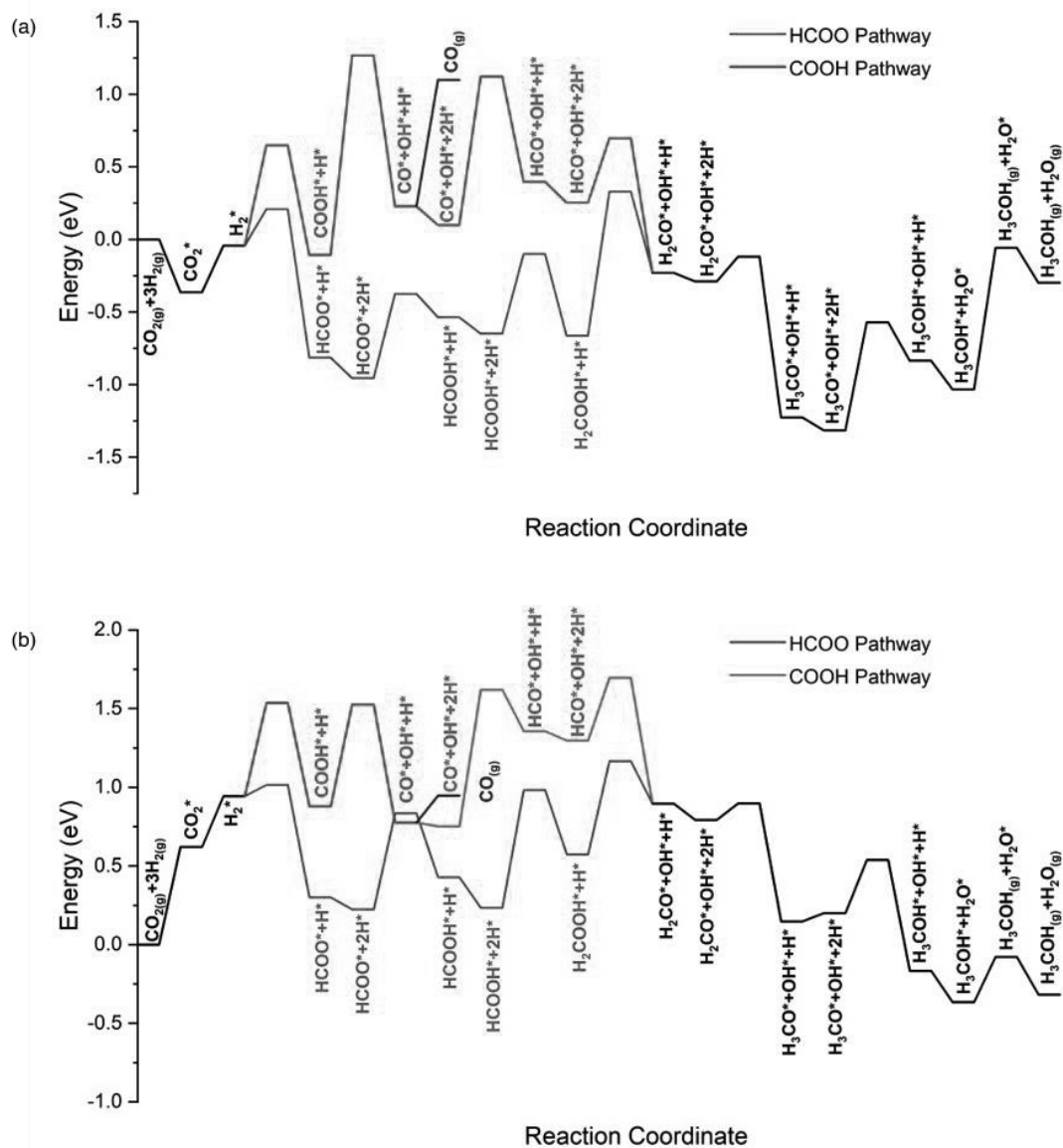
Figure 3-Free energy profile showing different pathways for \text{CO}_2 hydrogenation to methanol on the (a) \text{ZrO}_2/\text{Cu} interface and (b) \text{ZnO}/\text{Cu} interface of the \text{Zr}_1\text{Zn}_2\text{O}_3/\text{Cu} (111) catalyst model obtained from DFT calculations. Green – HCOO pathway; Red – COOH pathway; Black – Common intermediates on both HCOO and COOH pathways; Blue – CO desorption in COOH pathway
