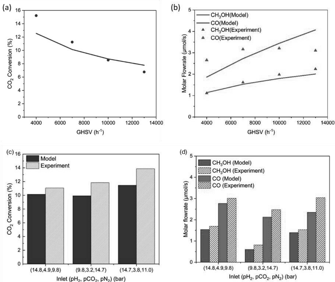
Figure 5- \text{CO}_2 conversion, reactor outlet molar flowrates as a function of (a,b) GHSV and (c,d) feed ratios. All these experiments/model data are measured/computed at P=30 bar. T=250\text{ }^{\circ}\text{C} , \text{GHSV}=7000\text{ h}^{-1} , inlet p\text{H}_2 , p\text{CO}_2 , p\text{N}_2=19.9, 6.7, 2.9 (bar) respectively, whenever it is not varied. Symbols and dashed columns represent experimental data points. Lines and solid filled columns represent microkinetic model predicted data points. Color codes: Blue- \text{CO}_2 conversion; Green, Red- reactor outlet \text{CH}_3\text{OH} , \text{CO} molar flow rates
