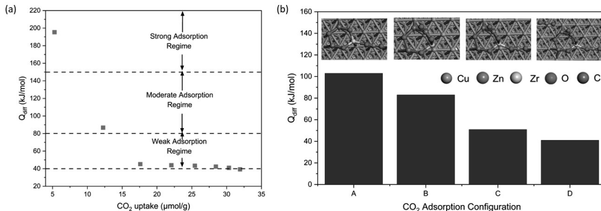
Figure 2-(a) Differential adsorption energy ( Q_{\text{diff}} ) of CO 2 on reduced Cu 2 Zn 1 Al 0.7 Zr 0.3 catalyst vs. CO 2 loading, obtained from microcalorimetric analysis. Red markers indicate experimental microcalorimetric analysis at different CO 2 uptake values. (b) DFT calculated differential adsorption energy of CO 2 on Zr 1 Zn 2 O 3 /Cu(111) catalyst with increasing CO 2 loading. The corresponding DFT structures are: (A) CO 2 on the ZrO 2 /Cu interface; (B) CO 3 on ZnO/ZrO 2 ; (C) CO 2 on ZrO 2 /Cu with pre-adsorbed CO 3 ; (D) Physisorbed CO 2 with pre-adsorbed CO 2 and CO 3 .
