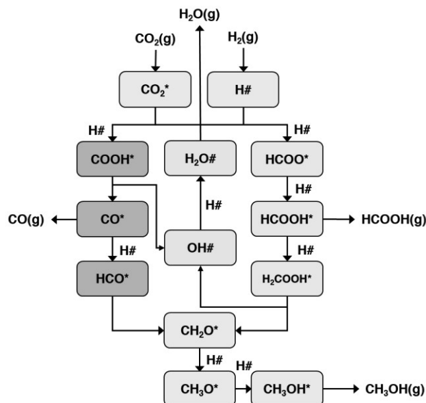
Figure 1: The schematic of the reaction network of \text{CO}_2 hydrogenation to methanol on the \text{Cu/ZnO/ZrO}_2 catalyst. The same set of reactions were considered to take place on both \text{ZrO}_2/\text{Cu} and \text{ZnO/Cu} interfaces. "*" (represents \text{ZrO}_2/\text{Cu} and \text{ZnO/Cu} sites) and "#" (represents pure \text{Cu} sites) indicate that the species is adsorbed on the surface. Colour codes: Green – Formate Pathway; Red – Carboxyl Pathway; Grey – Common Pathway; Blue – Water formation Pathway
