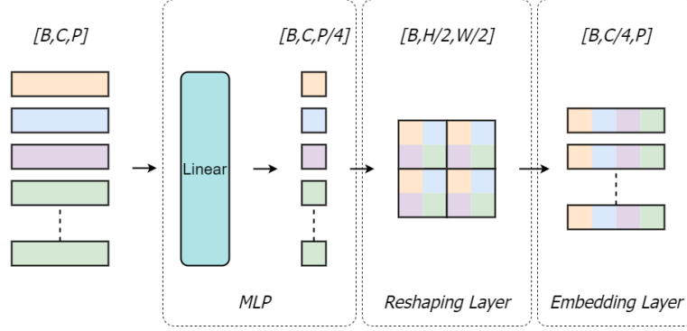
Fig. 2: Representation of the PPHR module. From left to right: example feature map derived from the image, patch representation of the image ( MLP block), linear transformation ( MLP block), patch representation of the image after linear transformation ( Reshaping layer ), patch reorganization ( Embedding layer ).
