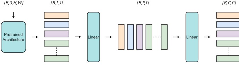
Fig. 1: From left to right: example feature map derived from the backbone pretrained Architecture, Liner transformation, second linear transformation after feature transpose.
