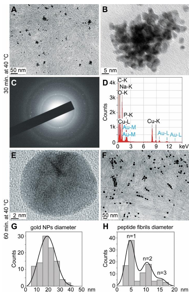
Figure 6. Study of AuNP formation within the hydrogel of 1 at 40 °C. A-D) During the first 30 minutes, polycrystalline AuNP clusters were found by TEM (A, B) and selected area electron
