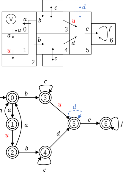
Fig. 1. A plan of a zone-controlled AGV and its corresponding automaton model with unobservable event u .
