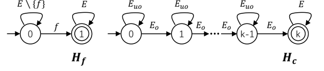
Fig. 4. H_f and H_c for conventional k -diagnosability.
