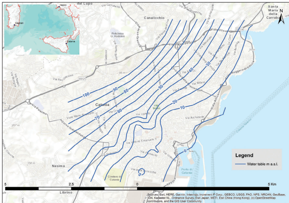
Fig. 18 - Water table map of the City of Catania (new original unpublished elaboration).
