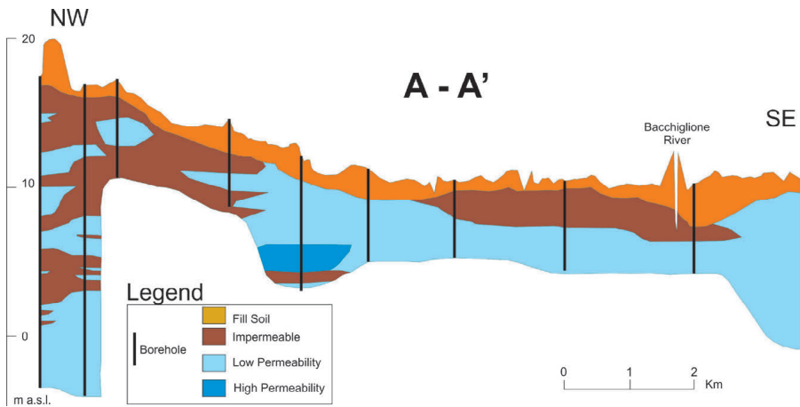
Fig. 7 - Hydrogeological cross section A-A' of Padova City (see Fig. 6).
