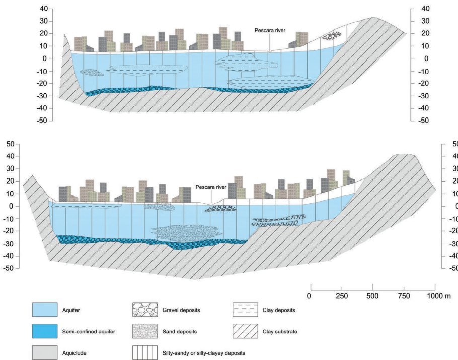
Fig. 14 - Schematica idrogeologica cross section of the urbanized area of Pescara, transversal to the river of the same name and parallel to the coastline. Above: structure in the western portion of the urbanized area about 3 km from the coastline. Below: structure about 1 km from the coastline.
