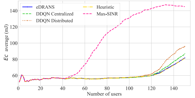
Fig. 12: Ec average for an incremental number of users.
