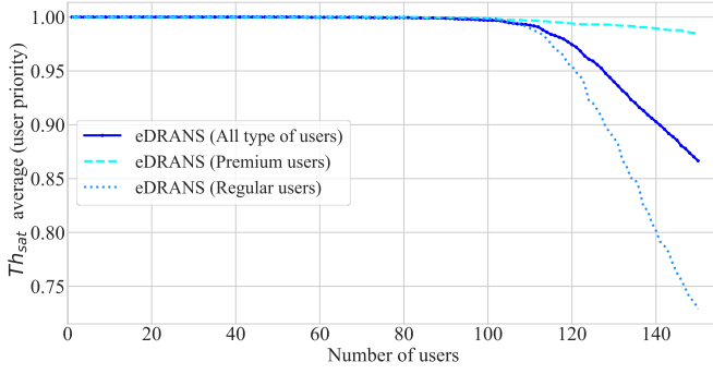
Fig. 9: Th_{sat} for different user priorities (eDRANS algorithm).
