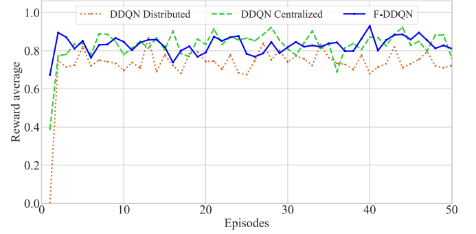
Fig. 7: Reward average during the training process.
