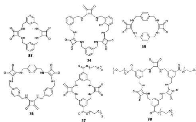
Fig. 12 Cyclic squaramide-based receptors featuring aryl spacers and in the cases of 37 and 38 also triethylene glycol monomethyl pendants via ester linkages.
