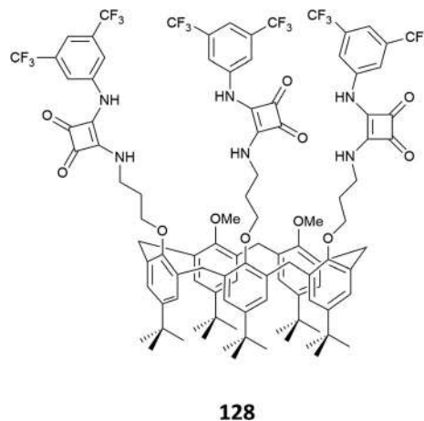
Fig. 45 Tris-squaramide 128 .
