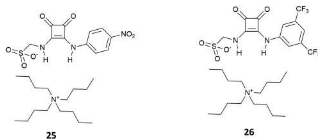
Fig. 6 SSA squaramides that are able to act as colorimetric sensors for H 2 PO 4 - .
