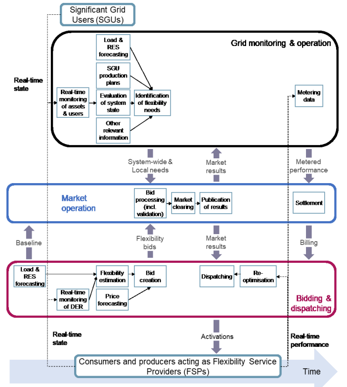
Fig. 2. Generic architecture for flexibility trading, with main blocks, activities and information exchanges.
