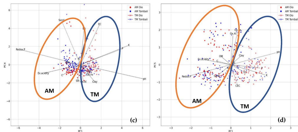
Figure A1. Biplot graphs for soil principal component (PC) combinations: (a) PC1 vs. PC2; (b) PC1 vs. PC3; (c) PC1 vs. PC4 and (d) PC1 vs. PC5.
