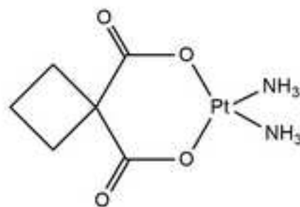
Carboplatin
