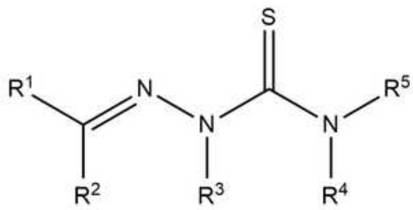
Thiosemicarbazones
