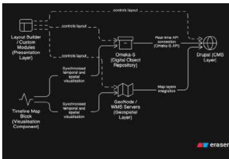
Figure 1. DOG system architecture schematic.
