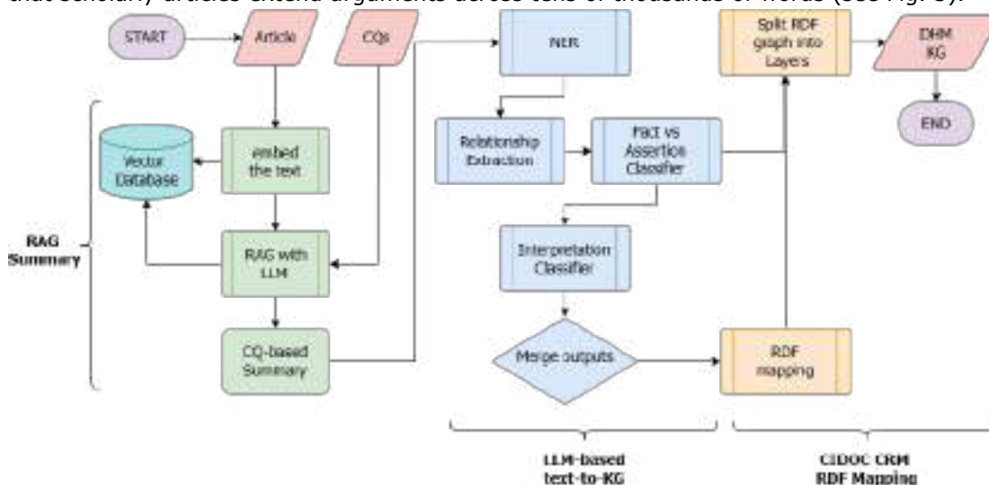
Figure 5. Pipeline Flowchart
