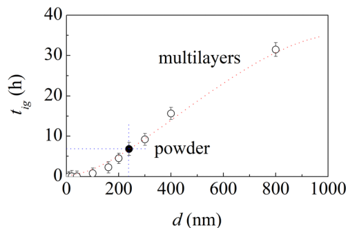
Fig. 4 The ignition time, t_{\text{ig}} , of multilayers (O) as a function of the bi-layer thickness, d . The vertical and horizontal dotted lines identify the ignition time of multilayers with d equal to 240 nm. The ignition time of the pristine Al–Ni powder mixture (●) is also shown. The dotted curve is a guide to the eyes.
