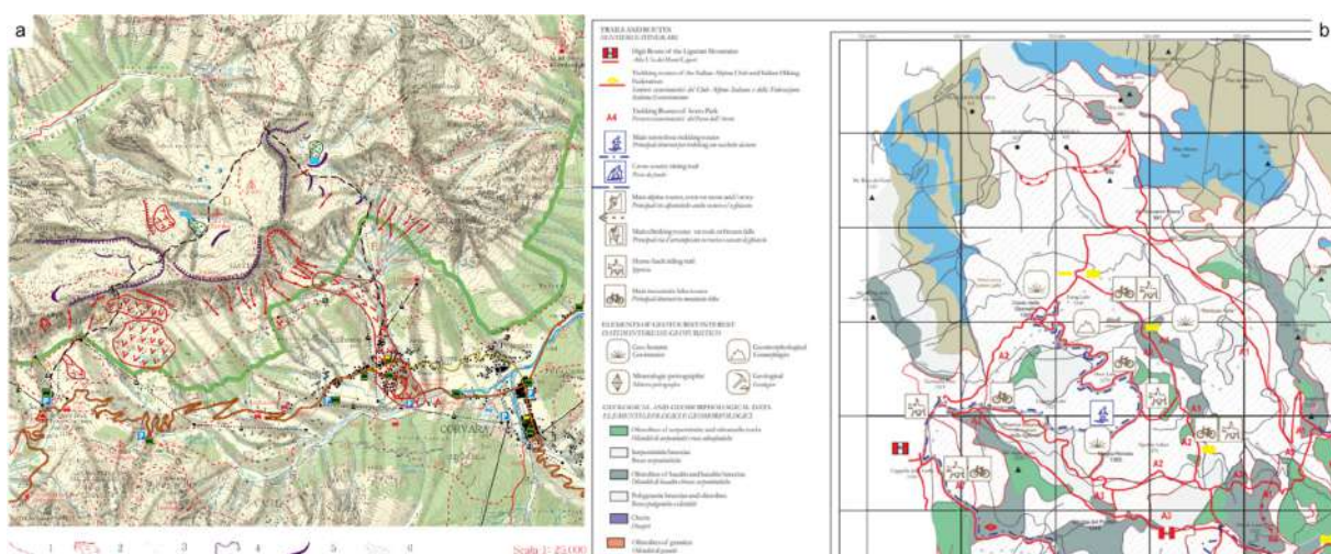
Figure 2. Examples of geotourism map for amateurs of Earth Sciences. (a) Excerpt from the leaflet of the geological-geomorphological itinerary in Val Badia (Dolomites, Italy [modified after 79]. (b) Excerpt from the Geo-hiking Map of the Mt. Penna and Mt. Aiona area (Aveto Natural Park, Italy) [modified after 80].
