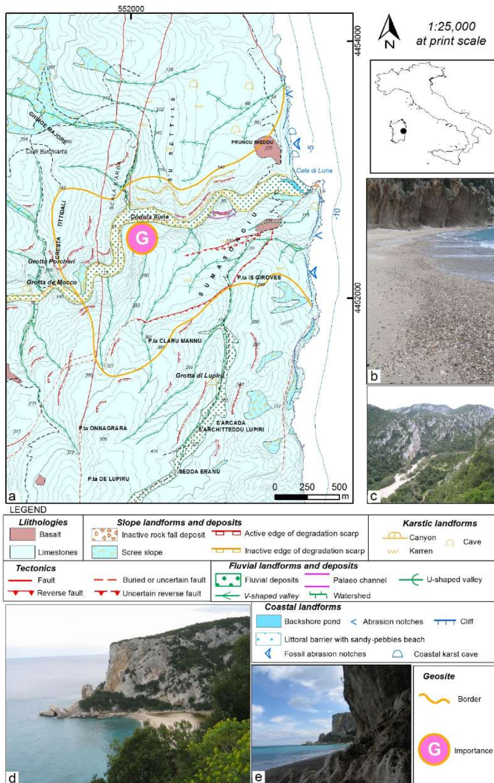
Figure 16. (a) Geomorphological map of the complex geomorphosite of Cala Luna. (b) View of sandy-pebbles beach and the littoral caves on carbonate cliff. (c) View from above of the Codula llune canyon. (d) Panoramic view of Cala Luna: cliff, backshore pond and beach. (e) Relic tidal notch and the Cala Luna cliff in the background.
