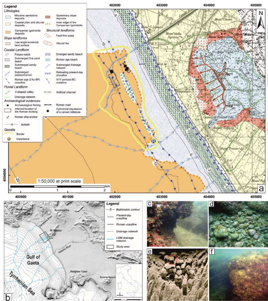
Figure 15. (a) Geomorphological map and location of the archaeological findings of the Sinuessa geosite; (b) location of the study area with reconstruction of the LGM drainage network. Pictures show several peculiar geomorphological and
