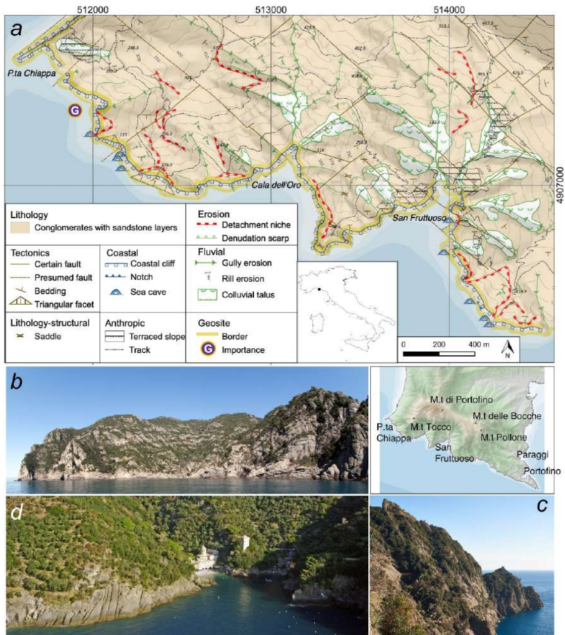
Figure 12. (a) Geomorphological map and location of the Portofino Promontory geosite, a composite and areal geosite characterized by high conglomerate sea cliffs. (b,c) Panoramic views of the southern slope of Portofino Promontory between Punta Chiappa and Cala dell'Oro, showing active sea cliffs with heights that exceed 100 m a.s.l.; (d) San Fruttuoso hamlet bay surrounded by ancient dry-stone walls agricultural terraces, built just over the edge of conglomeratic sea cliff.
