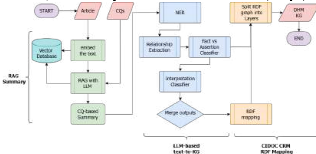
Figure 5. Pipeline Flowchart
