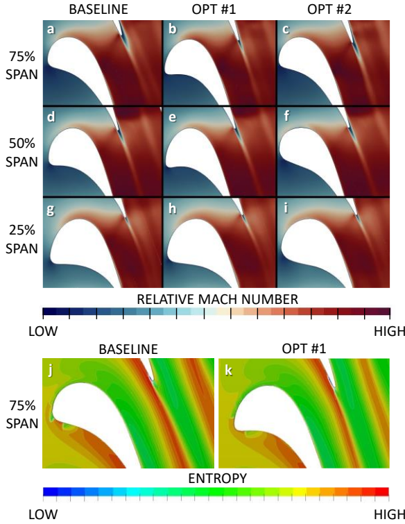
Figure 11: Flow-field visualization with relative Mach number contours for all the designs (a-i) and entropy contours for the baseline and OPT#1 (j, k) at constant-span sections. Pictures distorted.
