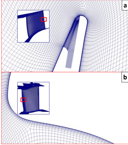
Figure 3: PADRAM Computational grids on the baseline geometries for the HPS (a) and HPR (b). The pictures show both full views of the surface meshes as well as blade-to-blade sections zooming in on the boundary layer mesh - Pictures distorted and not to scale.
