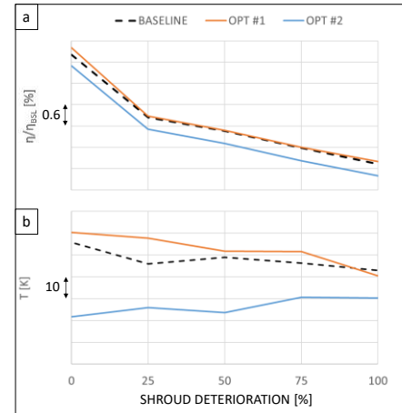
Figure 15: Effects of the shroud deterioration levels displayed in Fig. 6a on efficiency non-dimensionalized w. r. t. the baseline value (a) and peak HPR temperatures (b) on the designs under study.
