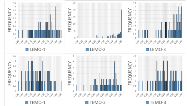
Figure 7: Frequency distributions for some of the parameters (LEMO and TEMO) obtained through uncertainty quantification on the design parameters of section 2.2 – suffixes -1, -2 and -3 respectively indicate section S1, S2, or S3 (see Figure 2).
