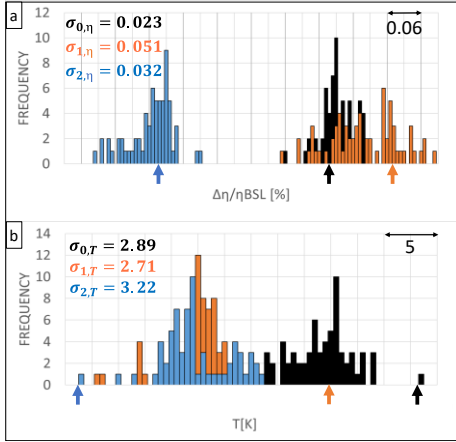
Figure 16: Frequency distributions of efficiency non-dimensionalized w. r. t. the baseline value (a) and peak HPR temperatures (b) after propagation of the noise space depicted in Fig. 7 on airfoil design parameters, for the designs under study: Baseline (black), OPT#1 (orange) and OPT#2 (blue). Vertical arrows indicate the unperturbed values. Standard deviations are also displayed.
