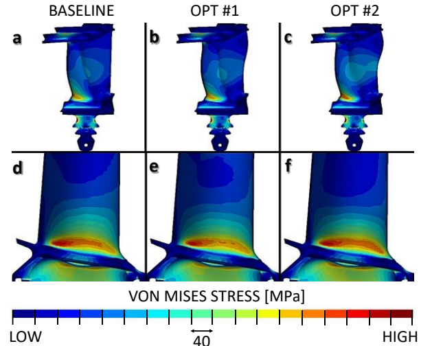
Figure 13: Von Mises stress contours on the different designs - frontal views (a, b, c) and lateral views showing the suction side hub fillet area on the three cases (d, e, f). Pictures distorted.
