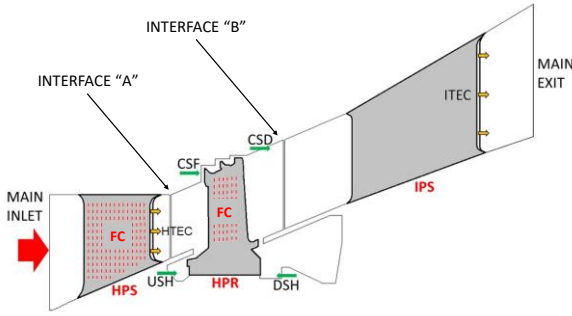
Figure 1: Schematic of the multi-row computational domain for the aerothermal simulations. Film cooling (FC) strip models are indicated with dashed red lines, acronyms can be found in nomenclature - Picture distorted and not to scale.
