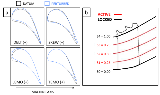
Figure 2: Design parameters used on the HPR geometry at each control section (a). The baseline shape is shown in black and the effect of applying each parameter to the section is shown in blue. (b) Active control sections are shown in red, "locked" control sections, where parameters are set to zero, are shown in black.
