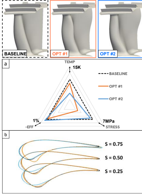
Figure 9: Frontal views of the baseline and optimal HPR geometries following the same nomenclature of Fig. 8. Objective function values are displayed in the triangular plot (a). Constant-span sections are shown in (b) with the same coloring scheme. Pictures representing the geometries are distorted.
