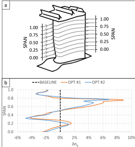
Figure 10: Spanwise isentropic efficiency calculation for the baseline and optimal designs. Schematic of the “constant-span streamlines” used to perform the calculation (a) – The plot in (b) shows the resulting streamline HPR isentropic efficiency deltas between each optimum and the baseline \Delta\eta_s = \eta_{s,OPT,i} - \eta_{s,BSL} .
