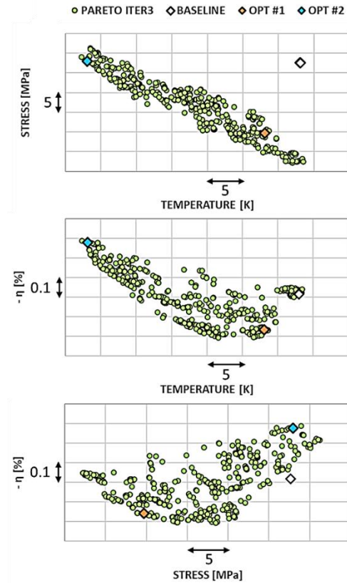
Figure 8: Final metamodel-predicted Pareto fronts of the multi-disciplinary optimization. The three-dimensional Pareto front is represented in bi-dimensional plots combining two objective functions at a time. Points corresponding to the baseline and two selected optima after CFD and FEM verification are included.
