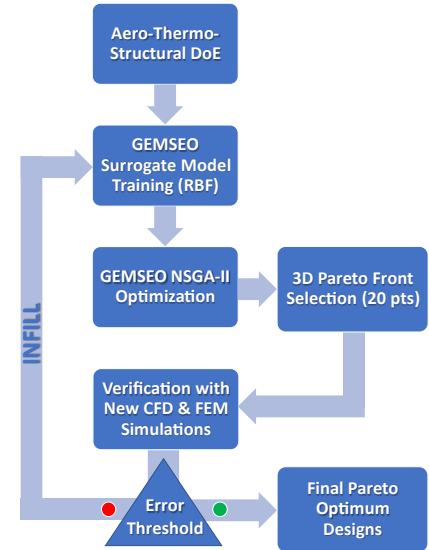
Figure 5: Optimization cycle workflow. The stopping/convergence criterion is the bottom center block “Error Threshold” where the non-dominated metamodels’ predictions are compared with CFD and FEM simulations and an error metric is calculated.
