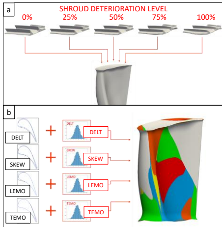
Figure 6: Modifications applied to the optimal designs to assess the designs' robustness to in-service deterioration in terms of shroud deterioration (a) and blade design perturbation (b) – Pictures distorted.
