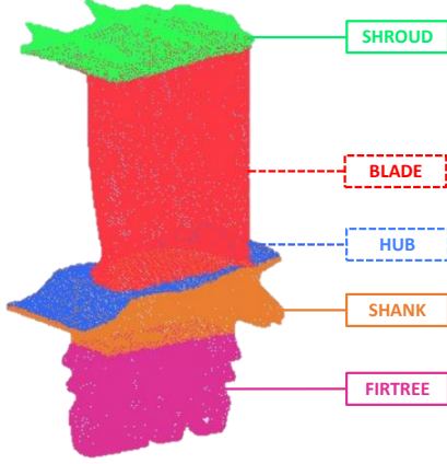
Figure 4: HPR structural mesh with components in different colors. Dashed lines indicate a morphing component whose geometry was imported from the aerothermal setup. Remaining parts were imported from CAD files - Picture distorted.
