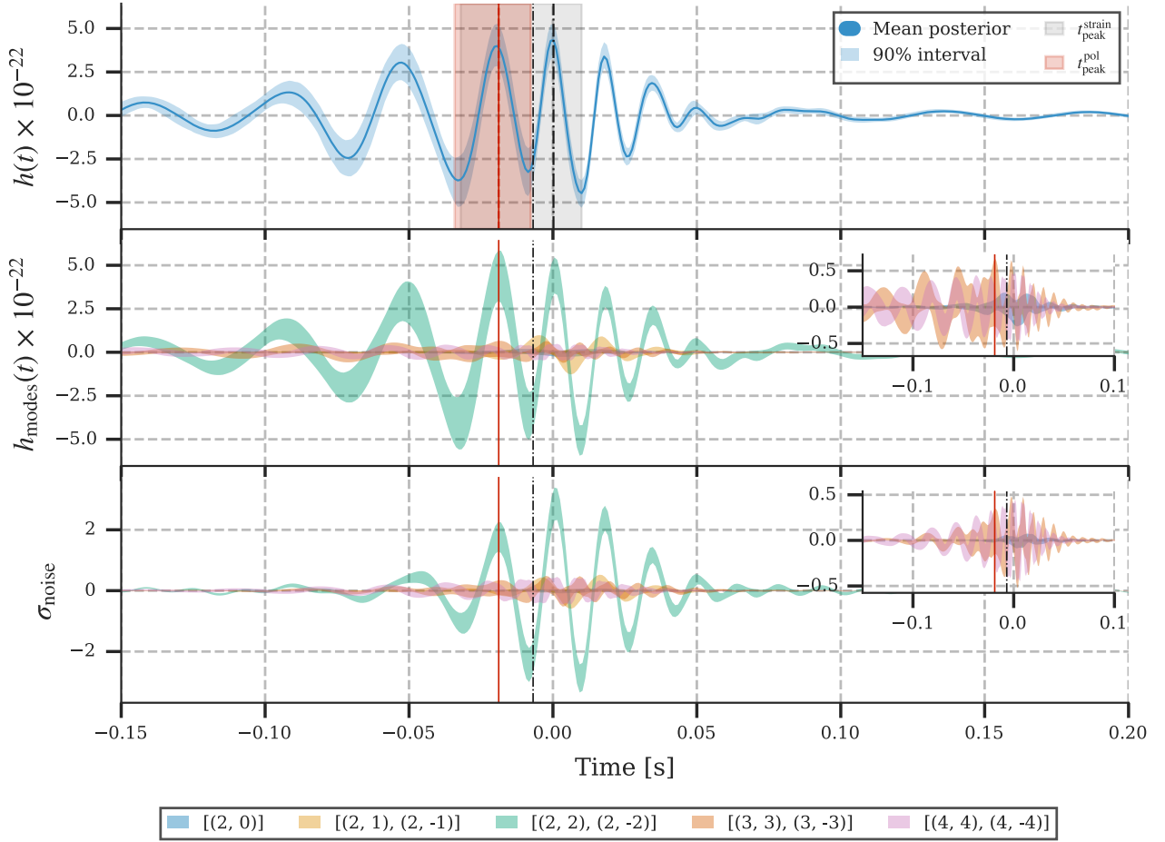
Figure 10. Top: posterior probability density functions of the NRSUR waveform time series, obtained via BILBY using the NRSUR waveform model at the LIGO Hanford detector. The red band shows the uncertainty in the measurement of t_{\text{peak}}^{\text{pol}} , and the gray band shows the uncertainty in t_{\text{peak}}^{\text{strain}} . Middle and bottom: posterior probability density functions of the mode strain, F_+h_+ + F_\times h_\times , with h_+ - ih_\times = -^2Y_{\ell,m}h_{\ell,m} + ^{-2}Y_{\ell,-m}h_{\ell,-m} , shown for the LIGO Hanford detector. The top part reports the unwhitened waveform, and the bottom part reports the whitened one, showcasing the impact of whitening in visualizing the signal morphology. The inset focuses on the (\ell, \pm m) = (2, 0), (3, 3), (4, 4) modes. The red line indicates the median of t_{\text{peak}}^{\text{pol}} , and the dashed-dotted black lines show the median of t_{\text{peak}}^{\text{modes}} .
