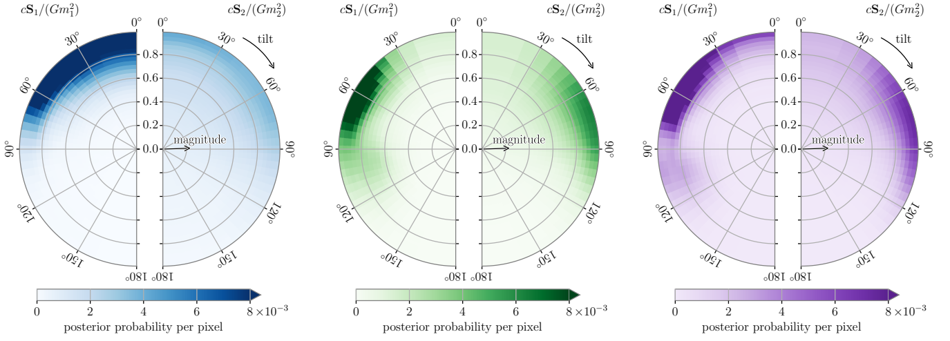
Figure 9. Posterior probabilities for the dimensionless component spins cS_1/(Gm_1^2) and cS_2/(Gm_2^2) , relative to the orbital angular momentum axis \hat{L} . From left to right, we compare the posterior probabilities obtained when analyzing LIGO Hanford data only (blue), LIGO Livingston data only (green), and a coherent analysis of LIGO Hanford and LIGO Livingston data (purple). In all cases, we show the posterior distribution resulting from equally combining samples from the five waveform models. The tilt angles are 0^\circ for spins that are aligned with the orbital angular momentum and 180^\circ for spins that are antialigned. Probabilities are marginalized over the azimuthal angles. The pixels have equal prior probability, being equally spaced over the spin magnitudes and the cosines of the tilt angles. The spin orientations are defined at a fiducial GW frequency of 10 Hz.
