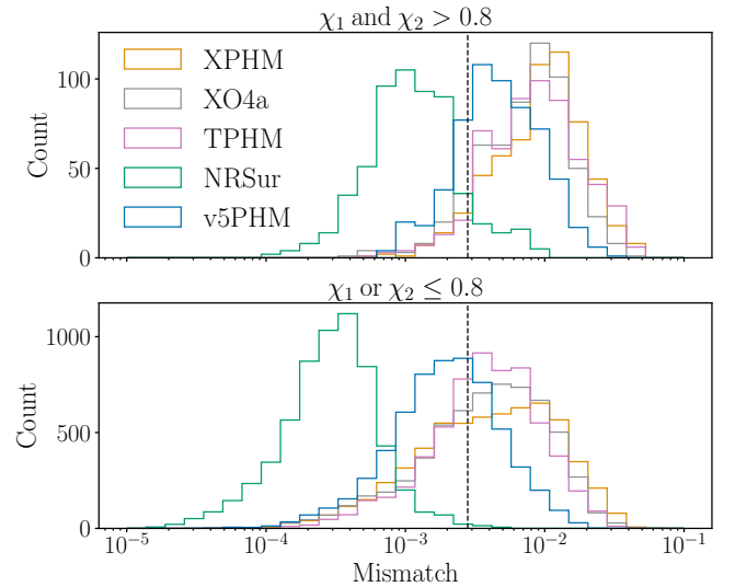
Figure 2. Mismatch accuracy of the waveform models considered in this Letter against 1123 NR simulations at a total mass of 300M_\odot and a range of inclinations between \iota = 0 and \pi/2 . The vertical dashed line at a mismatch of 0.0028 shows the conservative criterion discussed in the text.
