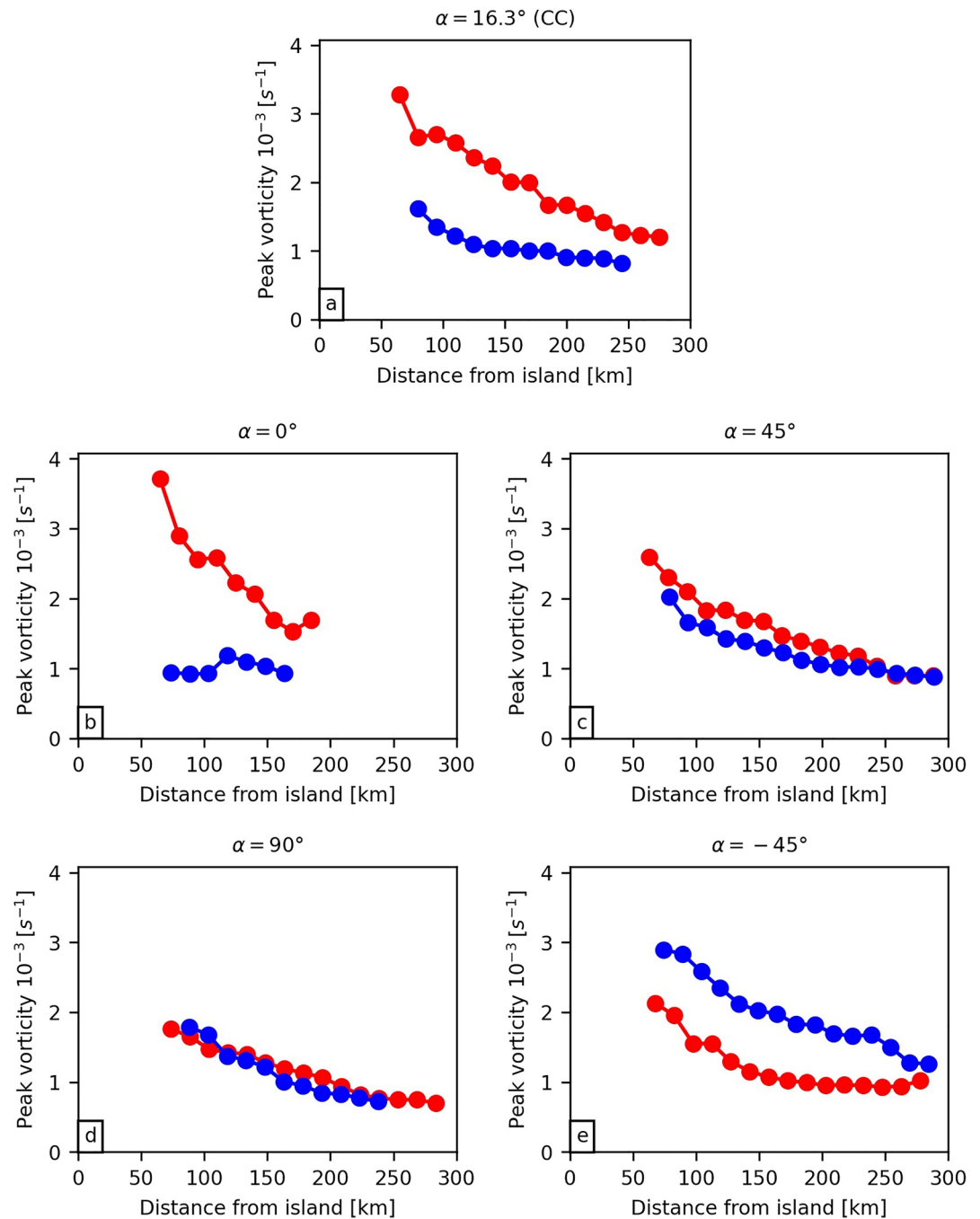
Figure 12. The absolute value of peak vorticity of cyclonic (red) and anticyclonic (blue) vortices plotted versus their distance from the island. Vorticity decay for the five different cases: control case (panel a) and the island rotations corresponding to \alpha = 0^\circ , 45^\circ , 90^\circ , and -45^\circ (panels b, c, d, e, respectively).
