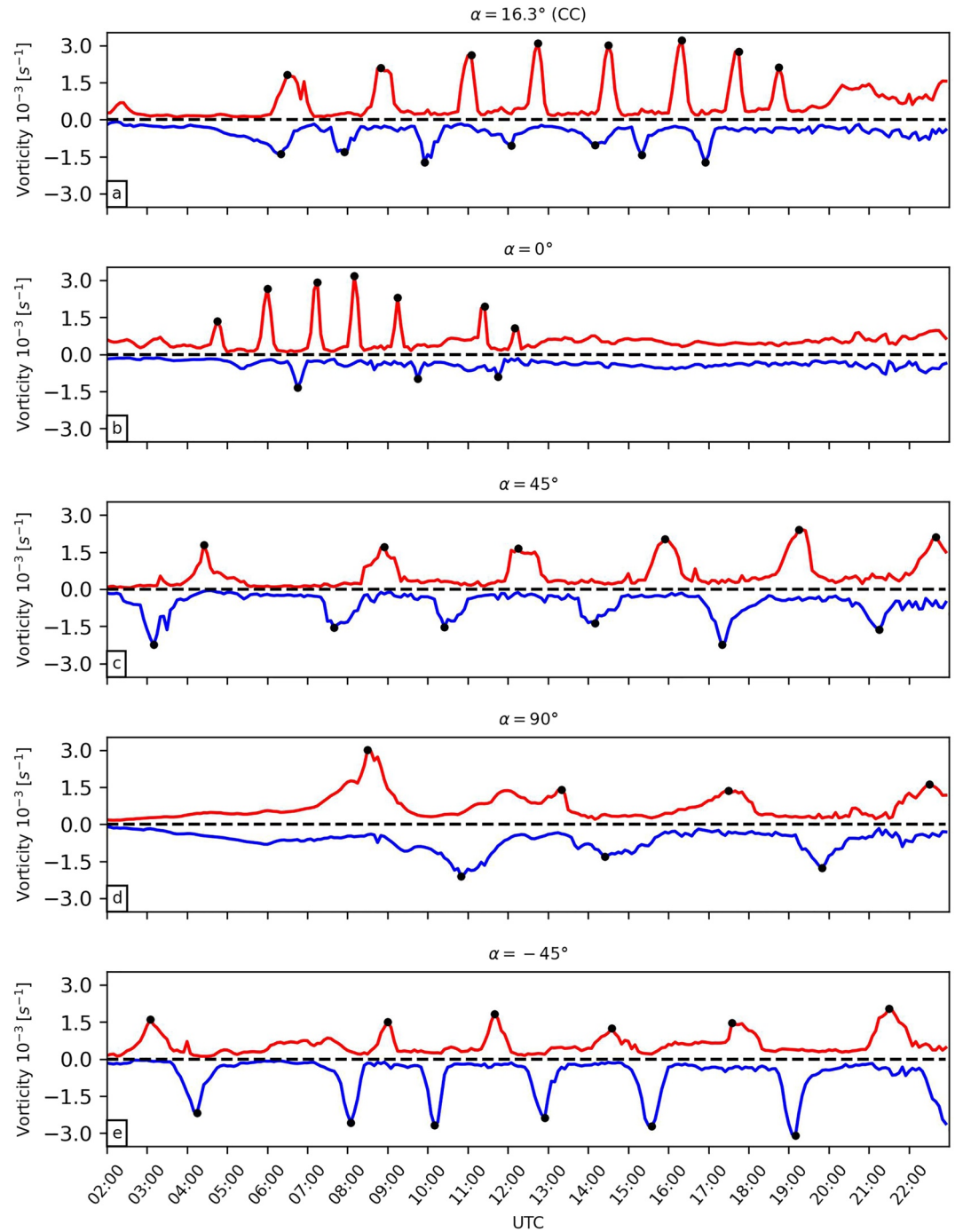
Figure 11. Maxima (red) and minima (blue) of vorticity computed along the section marked in Figures 2b and 7 versus time for the control case (panel a) and the island rotations corresponding to \alpha = 0^\circ , 45^\circ , 90^\circ , and -45^\circ (panel b, c, d, e respectively). The black points represent the local maxima and minima used to identify the timing of the vortex cores.
