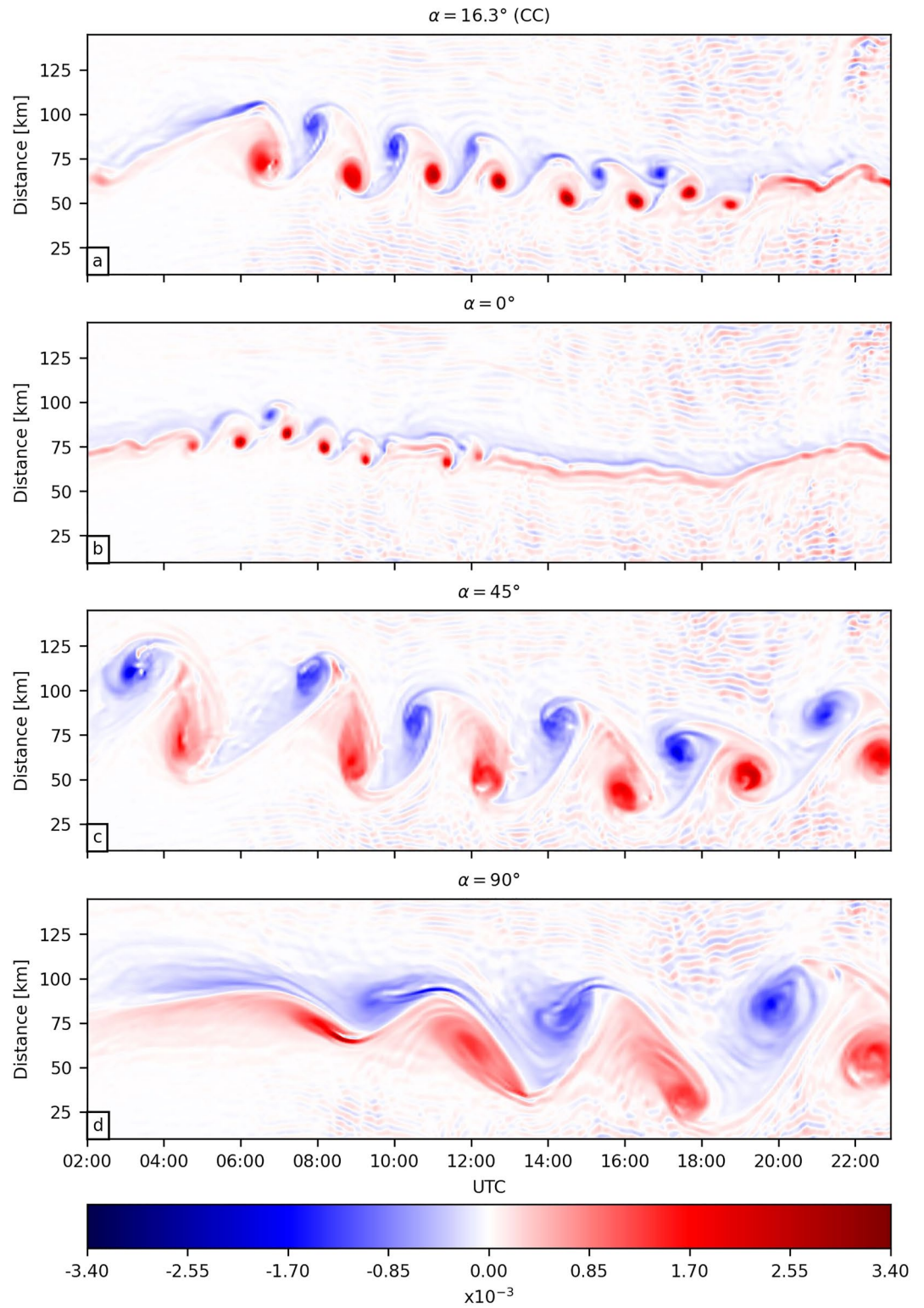
Figure 8. Hövmoller diagrams of vorticity ( \text{s}^{-1} ) computed along the cross-street section indicated in Figures 2b and 7 for the control case (panel a) and rotated orientations (panels b, c, d).
