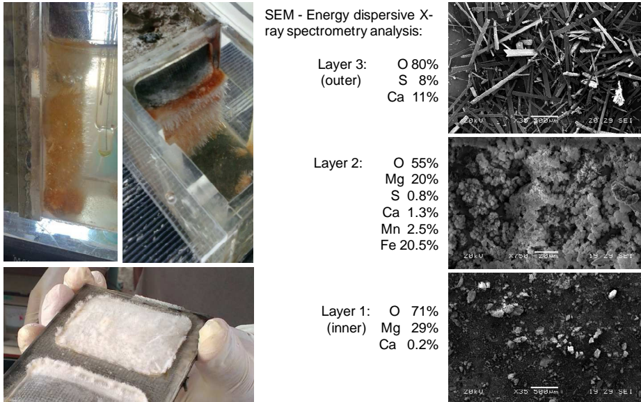
Figure 7 - Crystallization at the cathodic chamber after 43 days during the H 2 SO 4 test
