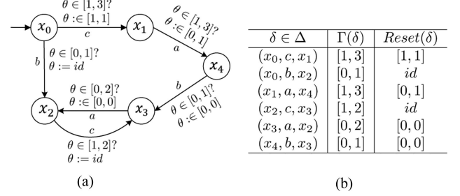
Fig. 1. TFA G w.r.t. the given timing function and clock resetting function. (a) TFA G . (b) Timing function and clock resetting function.
