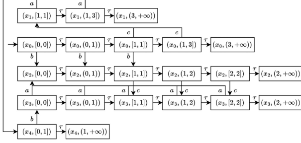
Fig. 2. Zone automaton G_z of the TFA G in Fig. 1.
