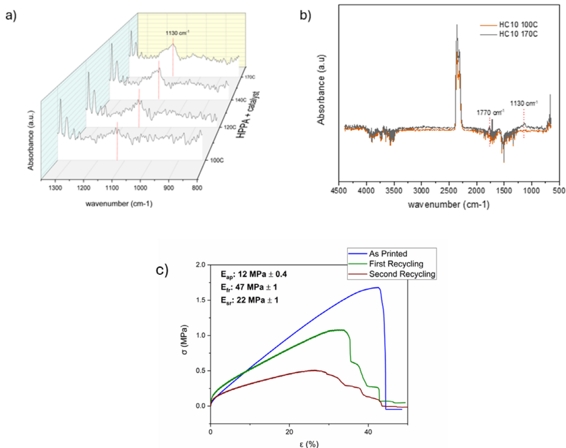
FIGURE 5 | a) TGA-IR analysis of HPPA + catalyst with peak formation at 1130 cm -1 with increasing temperature; b) TGA-IR analysis of HC10, with evidence of peaks at 1130 and 1770 cm -1 in the sample heated at 170°C; c) tensile test on thin films of HC10, printed, after the first thermal process and after the second thermal process.
