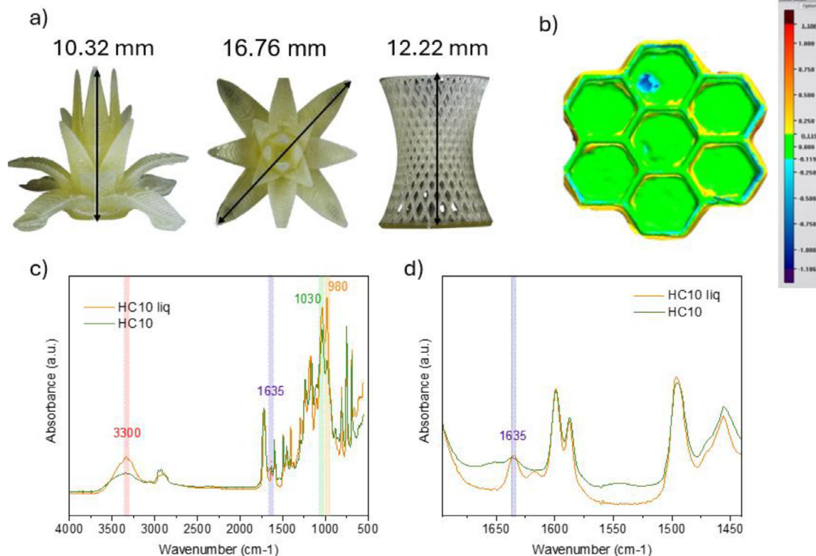
FIGURE 3 | a) examples of HC10 printed objects with complex geometries; b) 3D scanner of honeycomb printed with HC10 resin; c) ATR spectra comparison before and after phototopolymerization process, evidencing the peaks of interest; d) decrease of methacrylate peak at 1635 revealed by ATR spectroscopy.
