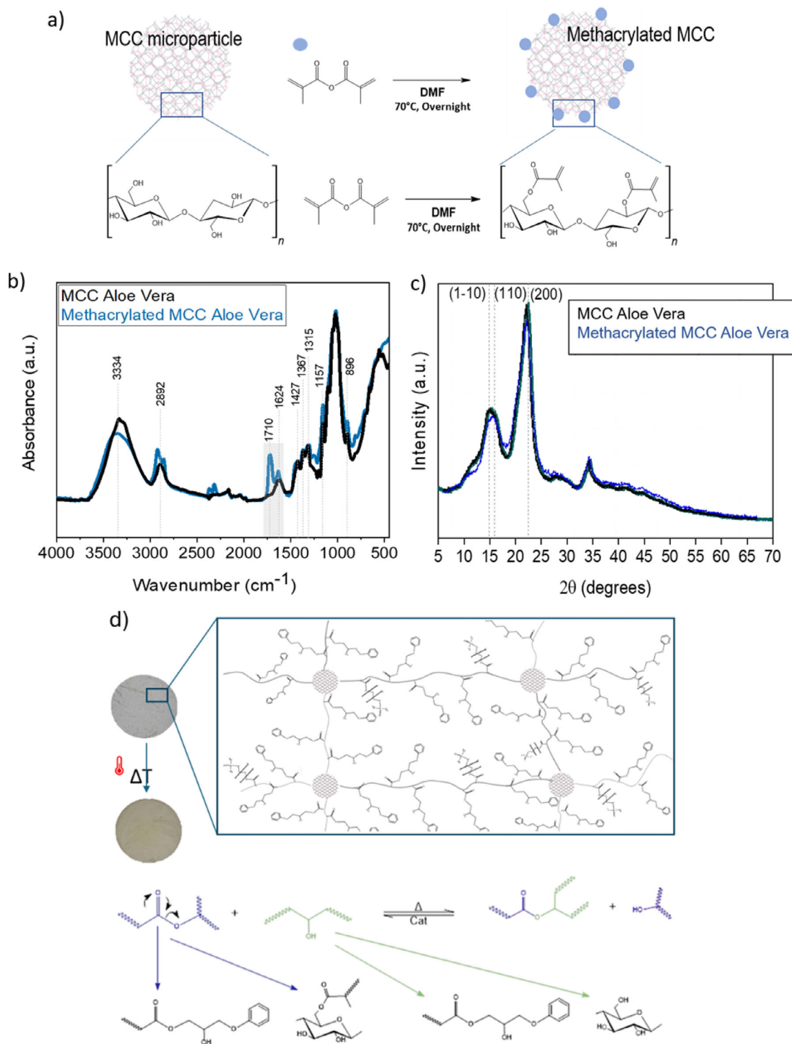
FIGURE 1 | a) Scheme depicting the MCC methacrylation process; b) FT-IR of the extracted MCC compared with the same after the methacrylation process; c) XRPD of the extracted MCC compared with the same after the methacrylation process; d) scheme of the polymer network and of the transesterification mechanism.
