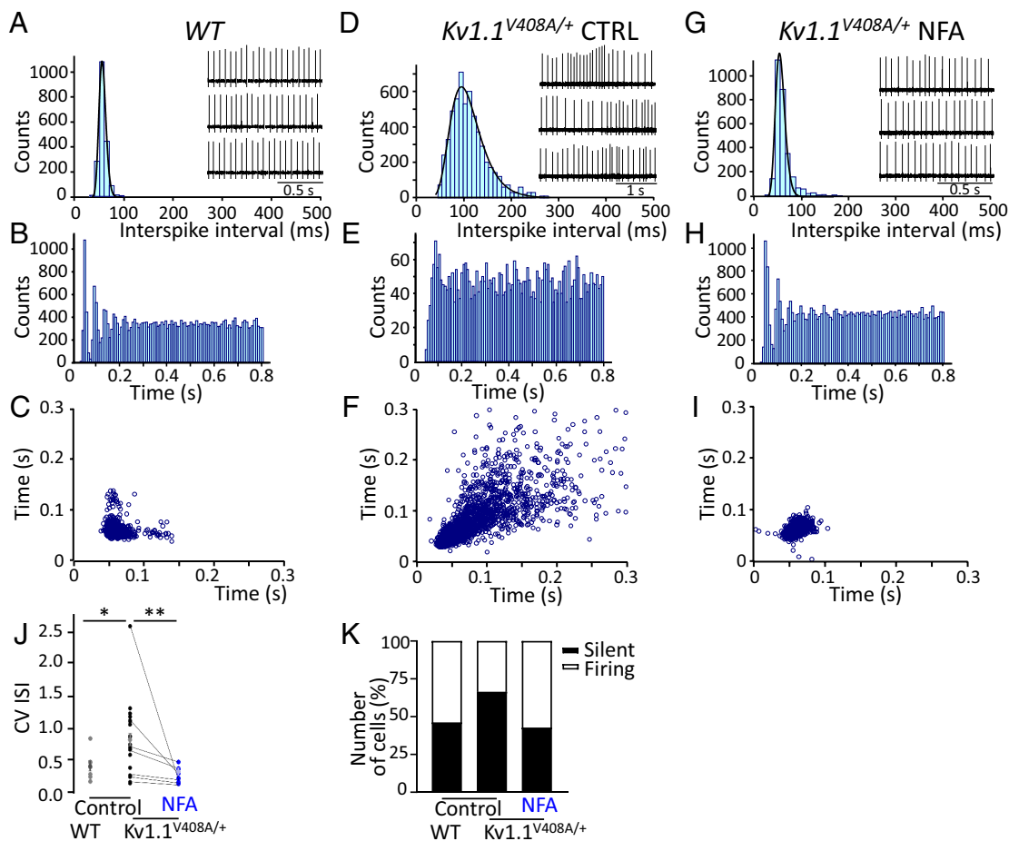
Fig. 4. NFA ameliorates the firing properties of Purkinje cells recorded from Kv1.1^{V408A/+} mice. Representative ISI distribution (A), spike recording ( Inset ), ISI autocorrelogram (B) and scatter plot (C) constructed for a PC recorded extracellularly from a cerebellar brain slice of a WT mouse and, respectively, for a sample Kv1.1^{V408A/+} PC recorded and analyzed before (Control, CTRL) (D–F), and after the superfusion of 100 \mu M NFA (G–I). Note that the ISI distributions were fitted with a probability density function of the exponentially modified Gaussian distribution with variance values of 8.7 for WT (A), 45 for Kv1.1^{V408A/+} /CTRL (D), and 15 after NFA treatment (G). (J) CV ISI calculated for WT and Kv1.1^{V408A/+} PCs (* P < 0.01 ; unpaired t test). The latter PCs were recorded before (Control) and after NFA (100 \mu M) application (mean \pm SEM; ** P < 0.001 ; unpaired t test). Note that Kv1.1^{V408A/+} PCs displayed an irregular firing compared to WT, which was ameliorated by NFA treatment. (K) Percentage of silent (black bar) or spontaneously firing (white bar) PCs recorded from WT and Kv1.1^{V408A/+} mice before (Control) and, upon incubation with NFA (100 \mu M). The NFA-induced increase in the percentage of spontaneously firing PCs was statistically significant: * P < 0.01 , ** P < 0.001 unpaired t test.
