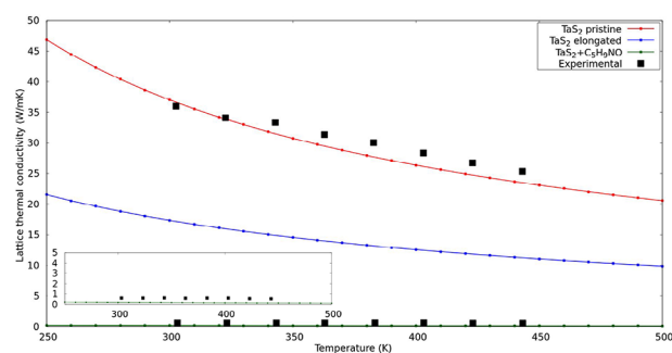
Figure 7. In-plane thermal conductivity of every system in respect of the temperature. The inset emphasizes the comparison between the estimated thermal conductivity and the experimental values for TaS 2 + C 5 H 9 NO.
