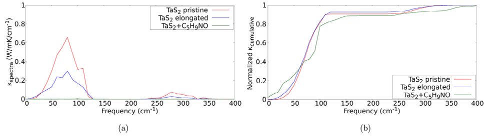
Figure 8. a) Thermal conductivity spectrum b) Cumulative thermal conductivity.
