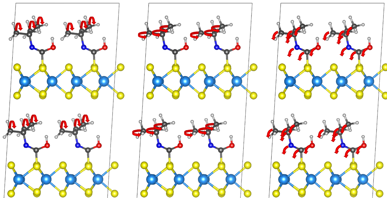
Figure 4. Red arrows visualize the atomic displacements associated with the, first, second, and third optical modes in the functionalized system TaS 2 + tert-butyl isocyanate.
