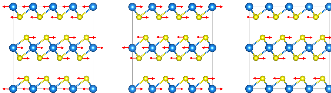
Figure 3. Red arrows visualize the atomic displacements associated with the, first, second and third quasi-acoustic modes in bulk TaS 2 .
