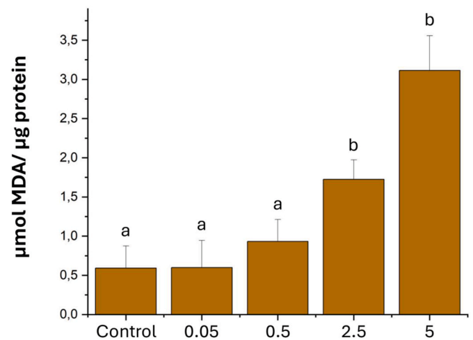
Fig. 3. Levels of lipid peroxidation (LPO) detected in samples of C. caespitosa exposed to different ash concentrations (Control; 0.05; 0.5; 2.5; 5 [g L -1 ]). Data are expressed as \mu\text{mol} of MDA per \mu\text{g} of proteins and as mean \pm SE ( n = 6 ). Lower-case letters indicate significant differences between corals maintained under different conditions ( p < 0.05 ).
