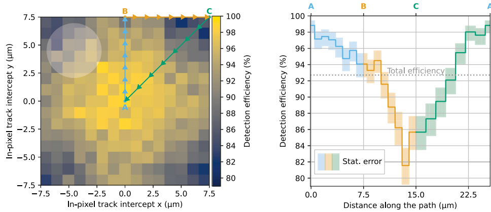
Fig. 17. In-pixel detection efficiency of a 10^{15} 1 MeV n_{eq} \text{cm}^{-2} irradiated sensor with threshold set to 160 e^- , measured with 10 GeV/c positive hadrons. The tracking resolution is represented by the white circle ( r = \sigma_{track} = 2.4 \mu\text{m} ) in the top left corner.
