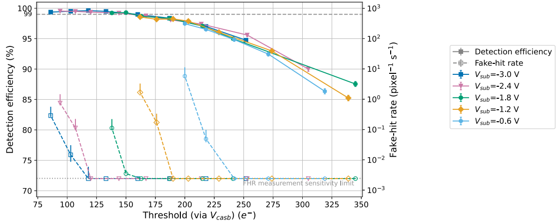
(a) Sensor irradiated to a dose of 10 kGy and 10^{13} 1 MeV n_{eq} \text{cm}^{-2} at different V_{sub} = V_{pwell} .
