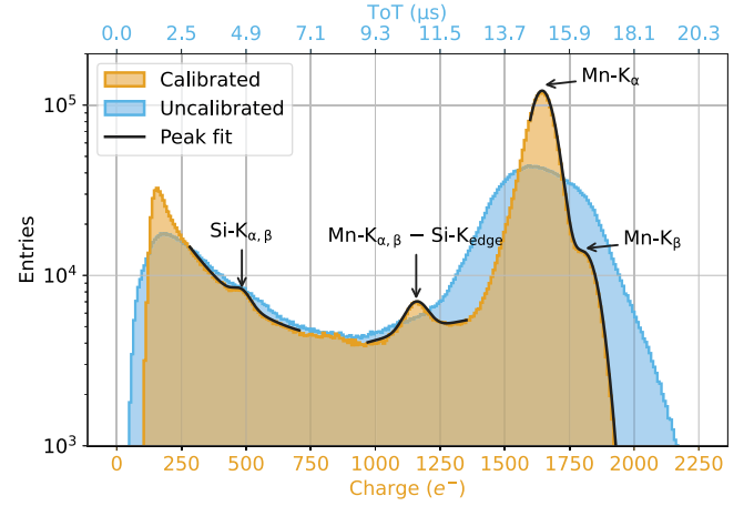
Fig. 13. Measured ^{55}\text{Fe} spectrum of single pixel clusters with a threshold set to 120 e^- . The initial spectrum (blue) is ToT calibrated (orange) which resolves the two x-ray peaks ( \text{Mn-K}_\alpha and \text{Mn-K}_\beta ) plus the \text{Mn-K}_{\alpha,\beta} escape ( \text{Mn-K}_{\alpha,\beta} - \text{Si-K}_{edge} ) and silicon fluorescence ( \text{Si-K}_{\alpha,\beta} ) peaks.
