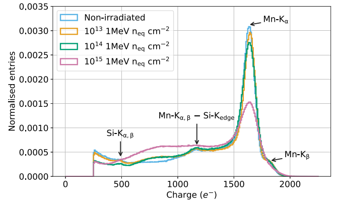
Fig. 14. Measured ^{55}\text{Fe} spectra of seed pixels for different levels of non-ionising irradiation: non-irradiated, 10^{13} , 10^{14} and 10^{15} 1 \text{ MeV } n_{eq} \text{ cm}^{-2} .
