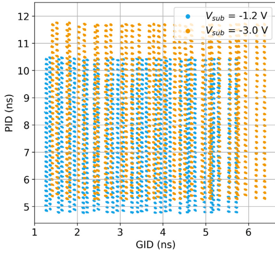
Fig. 12. The PID and GID data points corresponding to all pixels pulsed 100 times at V_{sub} = V_{puell} = -1.2 V and -3 V demonstrating the reverse bias dependence. Each cluster consists of 100 points and represents the measured PID and GID value for one pixel.
