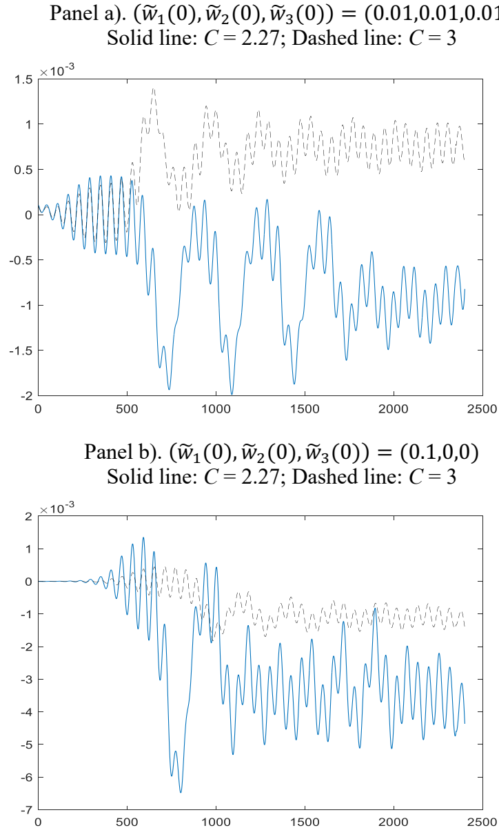
Figure 9. Paths of chaotic inflation. Higher-than-threshold C
