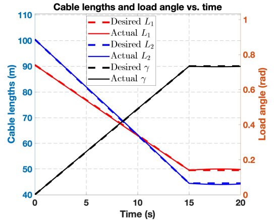
Fig. 3. Rope lengths L_1 , L_2 and load angle \gamma over time.
