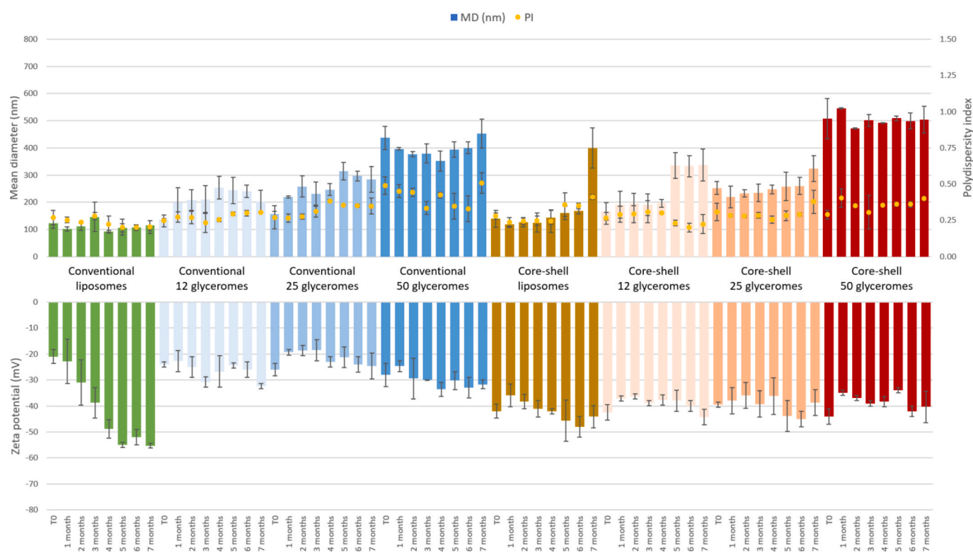
Fig. 2. Mean diameter, polydispersity index, and zeta potential of curcumin-loaded conventional and core-shell liposomes and glycosomes after preparation, 1, 2, 3, 4, 5, 6 and 7 months. Mean values \pm standard deviations, obtained from at least 3 measurements, are reported.
