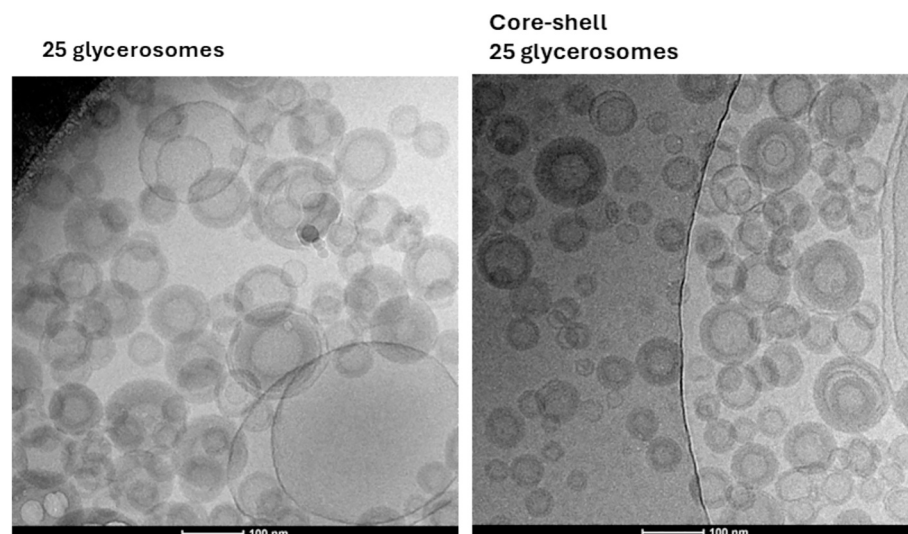
Fig. 1. Representative cryo-TEM images of conventional 25 glycosomes and core-shell 25 glycosomes.
