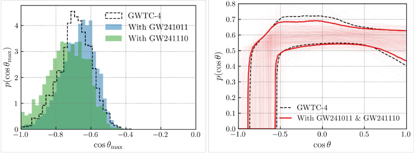
Figure 17. Right: inferred distribution of cosine spin–orbit misalignment angles, when additionally inferring the maximum misalignment angle (minimum \cos\theta value) among the binary black hole population (the MAX-TILT model). As in Figure 16, dashed lines indicate 90% credible bounds using black holes from GWTC-4.0 (A. G. Abac et al. 2025a), thick red lines indicate updated bounds when additionally including GW241011 and GW241110, and thin red lines illustrate individual draws from our updated population posterior. Left: posterior obtained on the minimum value \cos(\theta_{\max}) below which the \cos\theta distribution is truncated. The inclusion of GW241011 and GW241110 minimally affects inference of the maximum spin misalignment angle among the binary black hole population. Inference using GWTC-4.0 binary black holes requires \cos\theta_{\max} < -0.57 ( \theta_{\max} > 125^\circ ) at 90% credibility. Adding GW241011 and GW241110 gives \cos(\theta_{\max}) \leq -0.55 and -0.59 , respectively.
