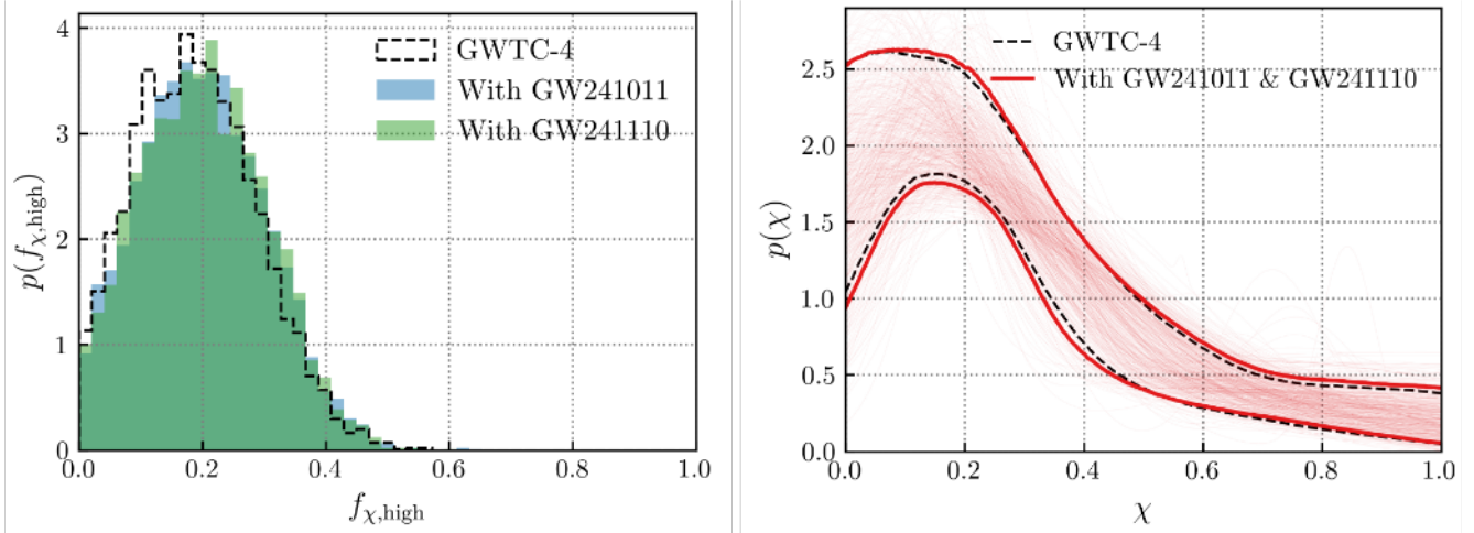
Figure 18. Right: inferred distribution of black hole component spin magnitudes when allowing for a distinct subpopulation of rapidly spinning black holes where one or both black hole components occupy this high-spin region (the HIGH-SPIN model). As above, the dashed lines and filled region span 90% credible bounds with and without GW241011 and GW241110, respectively. Left: inferred fraction of black holes comprising a possible highly spinning subpopulation. As above, results are negligibly affected by the inclusion or exclusion of GW241011 and GW241110. In both cases, current data do not require the existence of a distinct population of events with rapidly spinning components. When including GW241011 and GW241110, we bound f_{\chi,\text{high}} \leq 0.36 at 90% credibility, consistent with zero.
