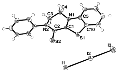
Figure 4. Molecular structure (ORTEP diagram) of [Ph 2 pipdt-C]I 3 (C = condensed; Ph-1C 3 ) showing the atom labeling scheme (corresponding selected bond lengths and angles are reported in Table 1). Thermal ellipsoids are shown at a 50% probability level. Additional data are provided in Section S5, Supporting Information.
