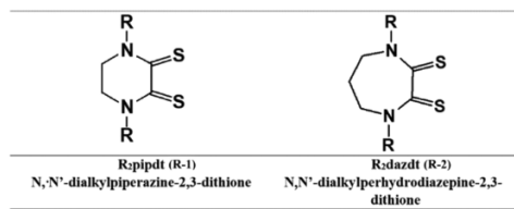
Chart 1. Cyclic Dithiooxamide Ligands of This Work
