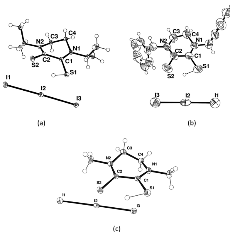
Figure 2. Molecular structure (ORTEP diagram) of {}^1\text{Pr-II}_3 (a), \text{Bz-II}_3 (b), and \text{Me-II}_3 (c) showing the atom labeling scheme. Thermal ellipsoids are shown at a 50% probability level. Additional data are provided in Section S5, Supporting Information.
