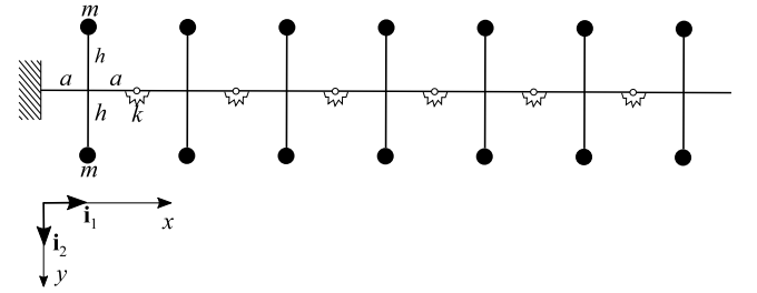
Fig. 4. Cross-beam.
