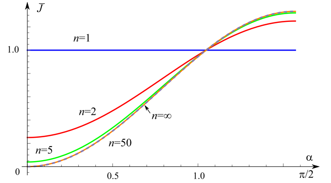
Fig. 3. Inertia parameter vs. \alpha . Here \bar{J} \equiv J/Ma^2n^2 and dashed curve relates to n \rightarrow \infty .
