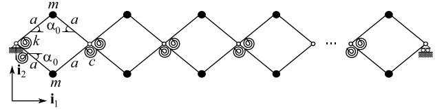
Fig. 6. Pantographic beam.
