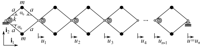
Fig. 1. Pantographic bar.
