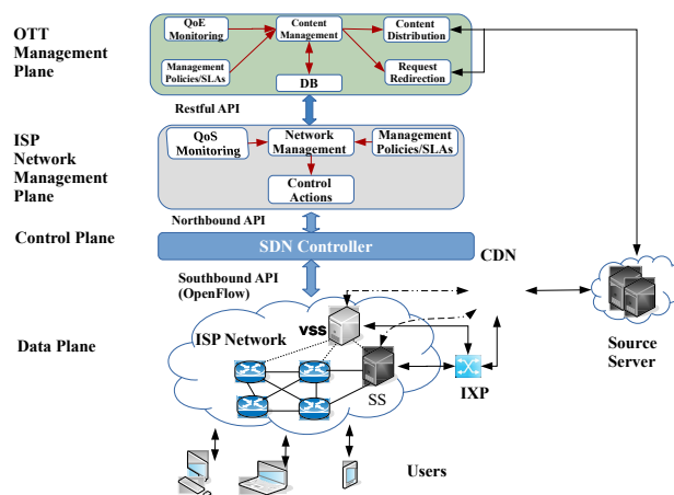
Fig. 17: Collaborative service QoE management by OTTP and ISP through SDN and NFV.
