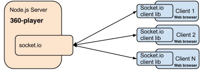
Fig. 1. Solution Architecture
