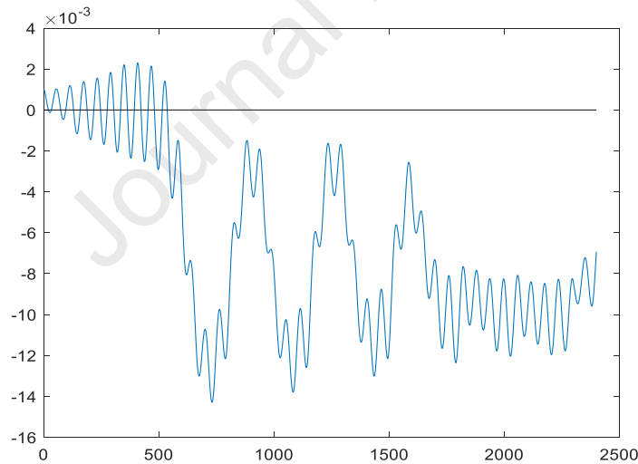
Figure 7. The moving average of chaotic inflation rate (window = 100 iterations).
