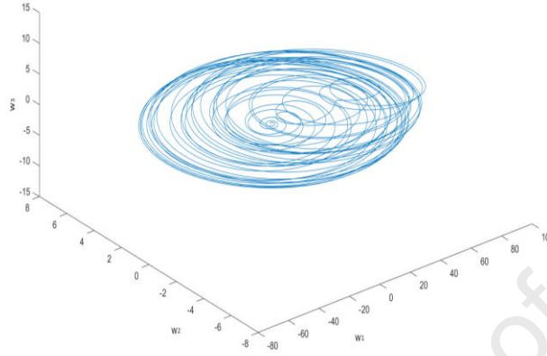
Figure 6. The chaotic attractor in the (\tilde{w}_1, \tilde{w}_2, \tilde{w}_3) space.
