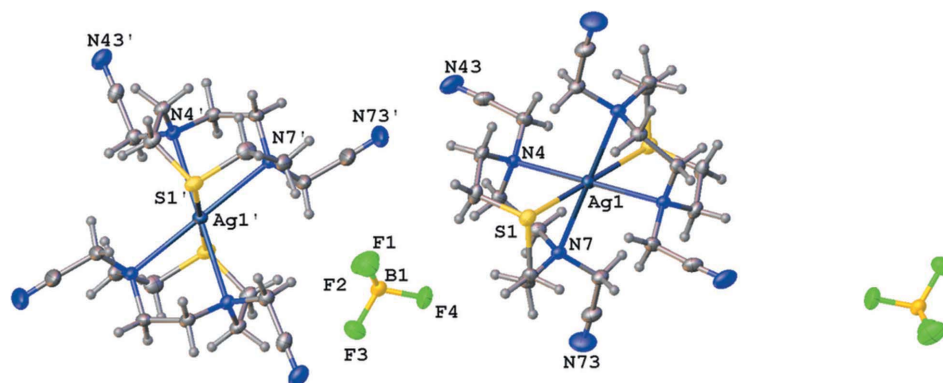
Figure 1 Two asymmetric units of complex [Ag(L 1 ) 2 ]BF 4 , showing the atom-numbering scheme. Displacement ellipsoids are drawn at the 50% probability level. The heteroatoms of the asymmetric unit are labelled.
