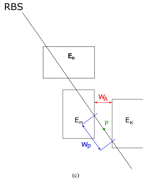
Fig. 6 – Definition of parameters for the COST 231 – Walfisch-Ikemi model. a) relevant to the definition of h_{\text{roof}} in the example h_{\text{roof}} = (h_1 + h_2)/2 . b) Definition and representation of the parameters b and \varphi . c) Representation of the two possible definition of the w parameter.
