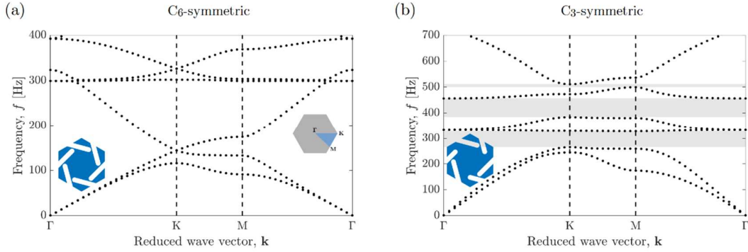
Figure 2: Band diagrams for the in-plane behaviour computed for (a) C_6 -symmetric and (b) C_3 -symmetric unit cells. Total band gaps are marked in grey. The occurrence of Dirac cones in the case of a C_6 -symmetric unit cell (a) is associated with the opening of band gaps in the C_3 -symmetric unit cell (b).
