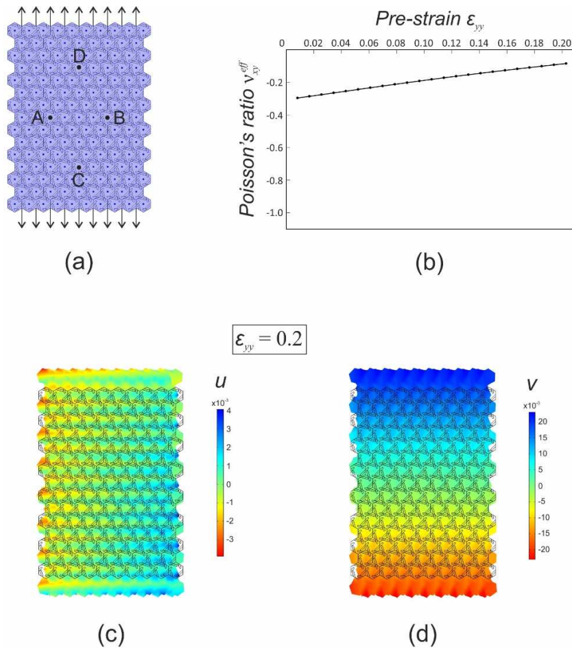
Figure C2: (a) Finite model, made of 10 \times 15 C_3 -symmetric cells and subjected to imposed displacements at the horizontal boundaries; (b) effective Poisson's ratio v_{xy}^{eff} versus the imposed engineering strain \epsilon_{yy} ; (c,d) displacement field components u and v , represented in colour scale.
