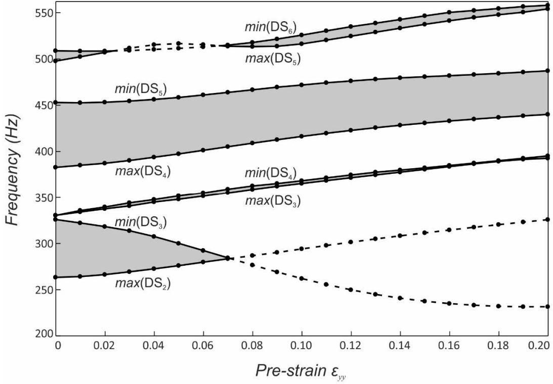
Figure 7: Frequency ranges of the lower band gaps (in grey colour) versus the imposed pre-strain \varepsilon_{yy} . The band gaps are determined by calculating the minima ( min ) and maxima ( max ) of the dispersion surfaces (DS), where the subscript refers to the number of the considered dispersion surface.
