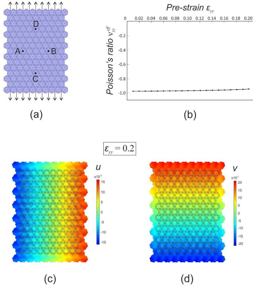
Figure C1: (a) Finite model, made of 10 \times 15 C_6 -symmetric cells and subjected to imposed displacements at the horizontal boundaries; (b) effective Poisson's ratio v_{xy}^{eff} versus the imposed engineering strain \epsilon_{yy} ; (c,d) displacement field components u and v , represented in colour scale. Fare clic o toccare qui per immettere il testo.
