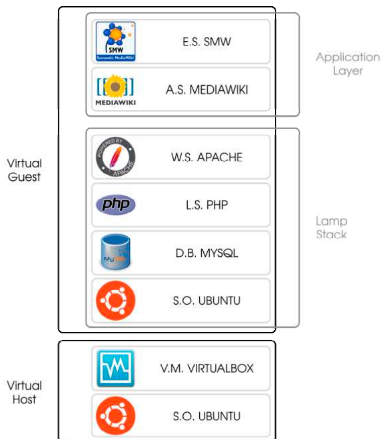
Figure 3. The software stack (simplified) of the KMS [39].
