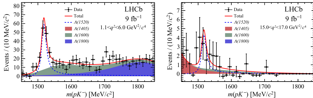
FIG. 2. Distribution of the pK^- mass, after background subtraction, for \Lambda_b^0 \rightarrow pK^-\mu^+\mu^- signal candidates in the (left) 1.1 < q^2 < 6.0 \text{ GeV}^2/c^4 and (right) 15.0 < q^2 < 17.0 \text{ GeV}^2/c^4 regions. Fit results are overlaid.
