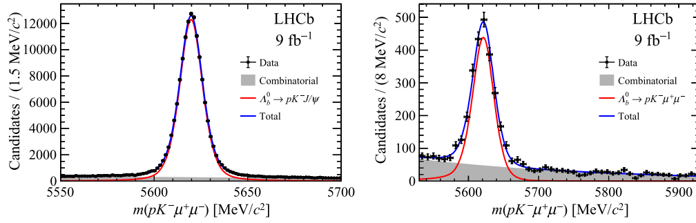
FIG. 1. Mass distribution for the (left) \Lambda_b^0 \rightarrow pK^-J/\psi and (right) \Lambda_b^0 \rightarrow pK^-\mu^+\mu^- , integrated over the considered q^2 intervals. Fit results are overlaid.
