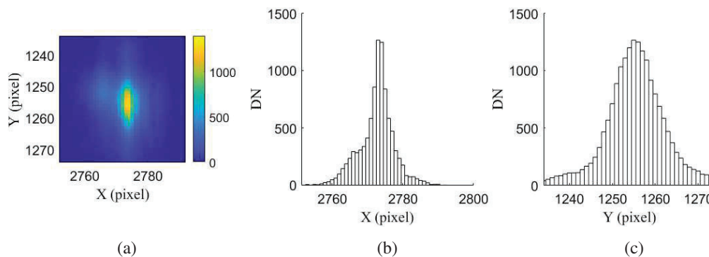
Figure 9. Example of color image (a) and x (spatial) (b) and y (spectral) (c) plots of an image spot at the HYPSONS spectrometer focal plane. This is the spectral projection of the 587.56 nm HeI line.
