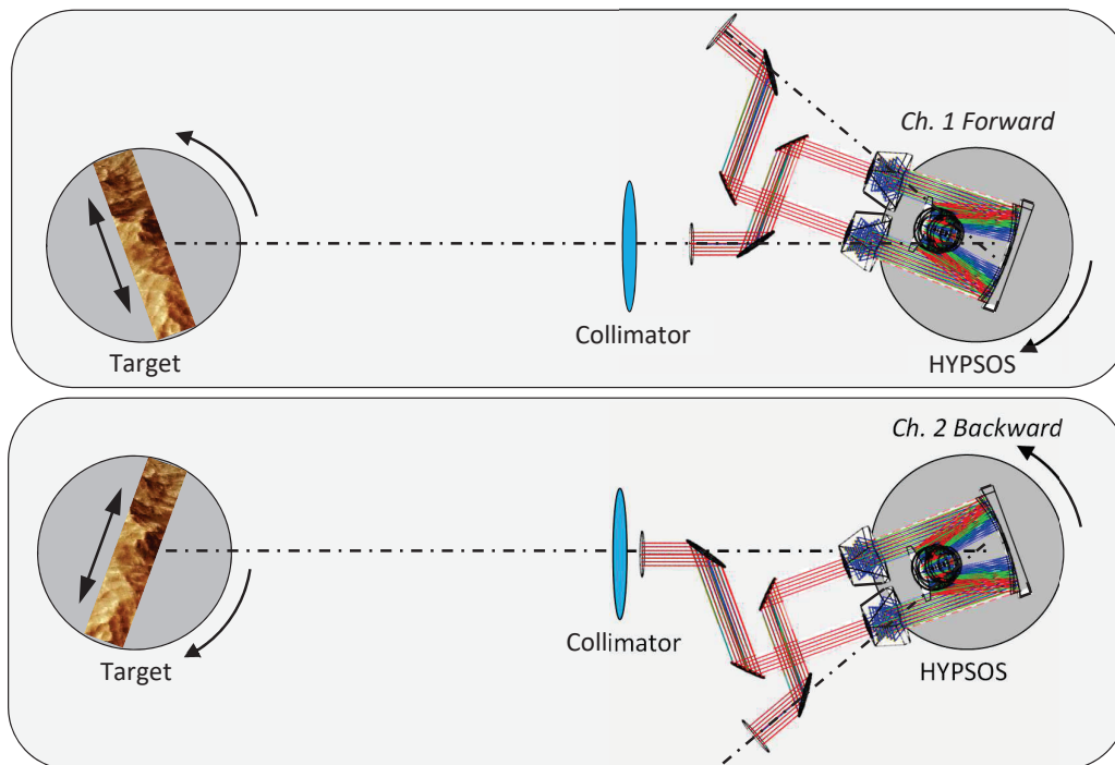
Figure 6. HYPOS acquisition configuration scheme. On top, the configuration for reproducing the acquisition with the forward channel is shown; on bottom, the same for the backward channel.
