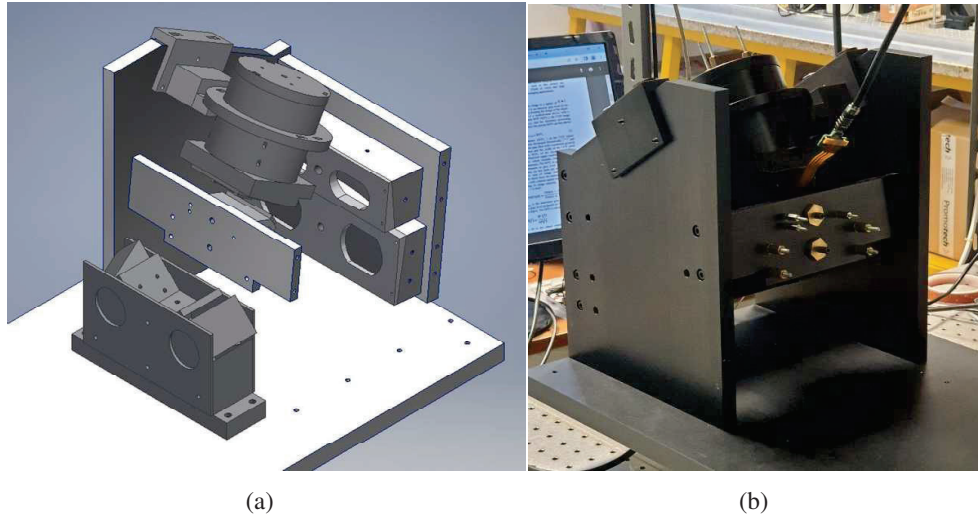
Figure 5. In (a) an open view of the rendered HYPSOS structure. In (b) the view of HYPSOS prototype (the SPP's are not yet mounted). The approximate envelope is 310 \times 310 \times 320 \text{ mm}^3 .
