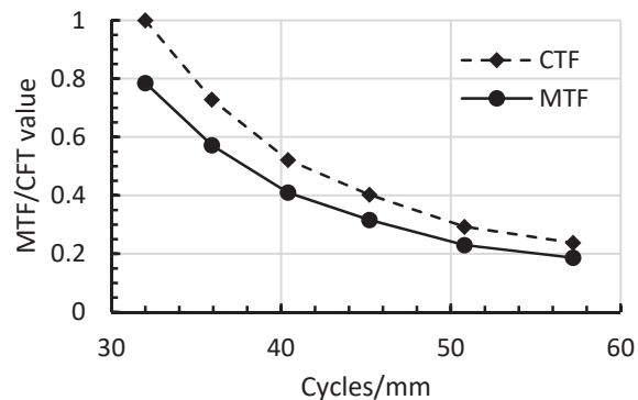
Figure 8. Estimate of the contrast (both CTF and MTF) on the HYPSONS telescope focal plane (right) by imaging a USAF target (left).
