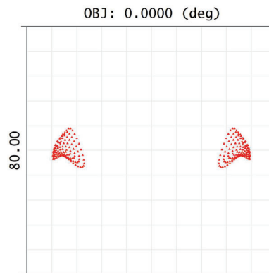
Figure 7. Ray tracing simulation of the spots on the telescope focal plane when illuminating HYPSONS with two on-axis collimated light beams, filling the two telescope apertures. The box has a size of 80 \mu\text{m} .
