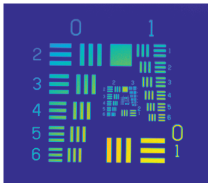
Figure 8. Estimate of the contrast (both CTF and MTF) on the HYPSONS telescope focal plane (right) by imaging a USAF target (left).
